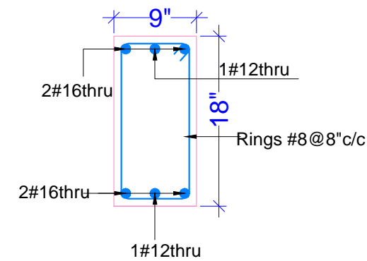
BEAM DETAIL
