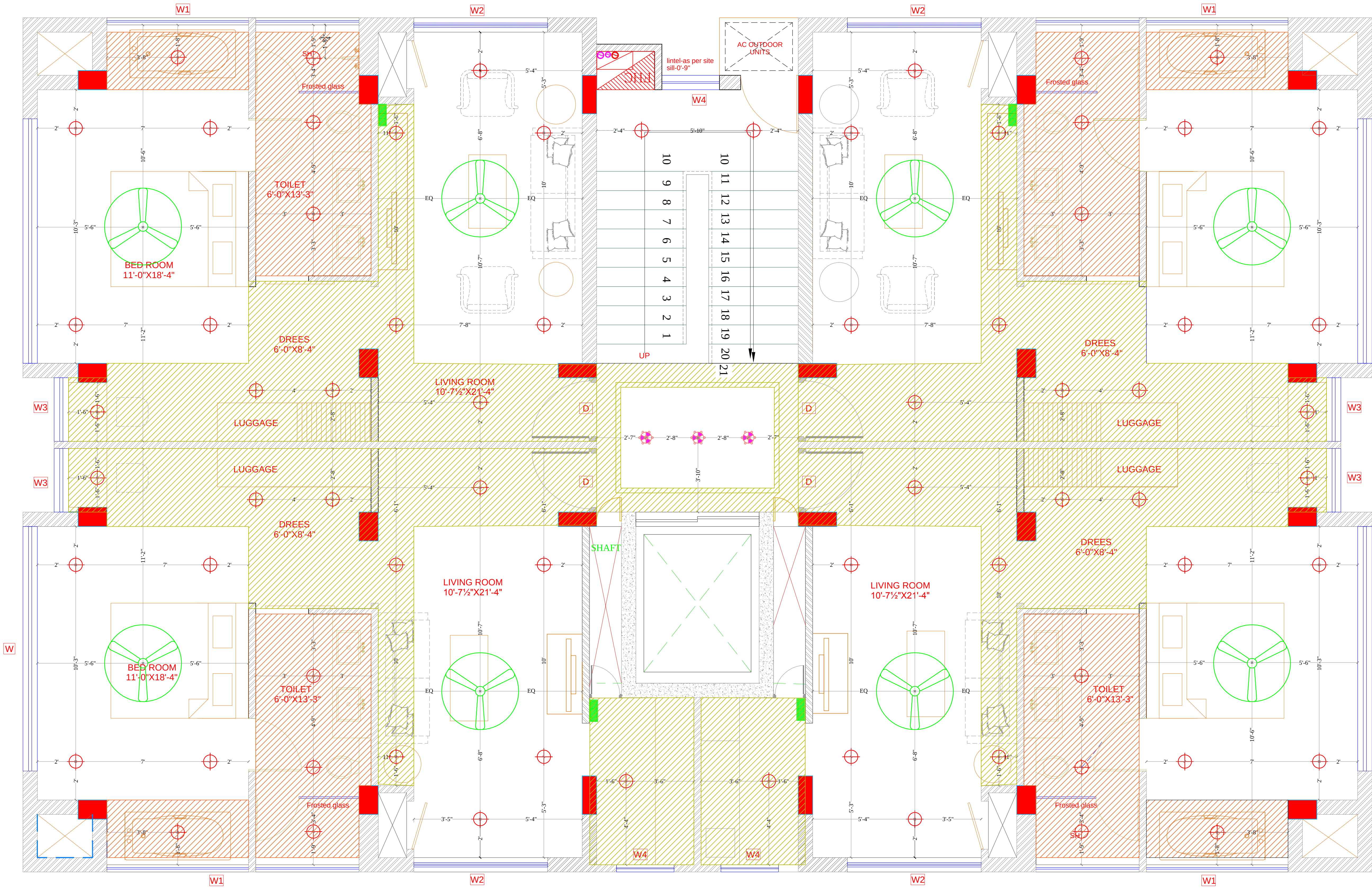
TYPICAL FLOOR CEILING ELECTRICAL
