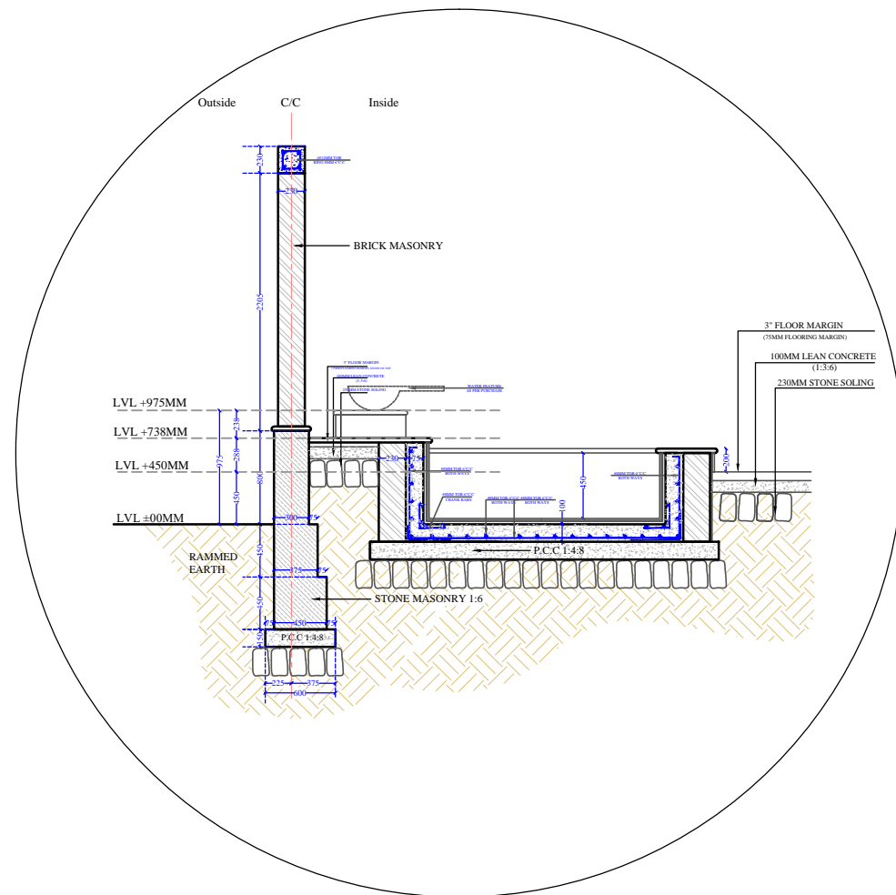
DETAIL AB 1
