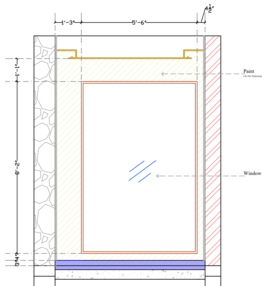
ELEVATION C
