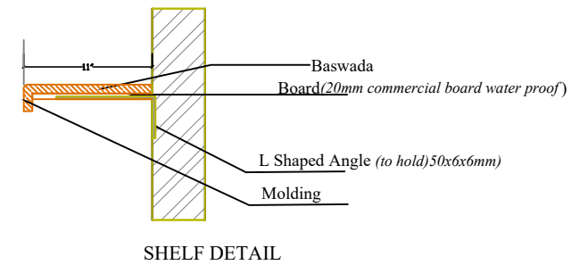
SHELF DETAIL
