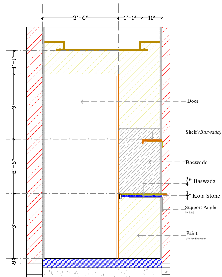
ELEVATION D
