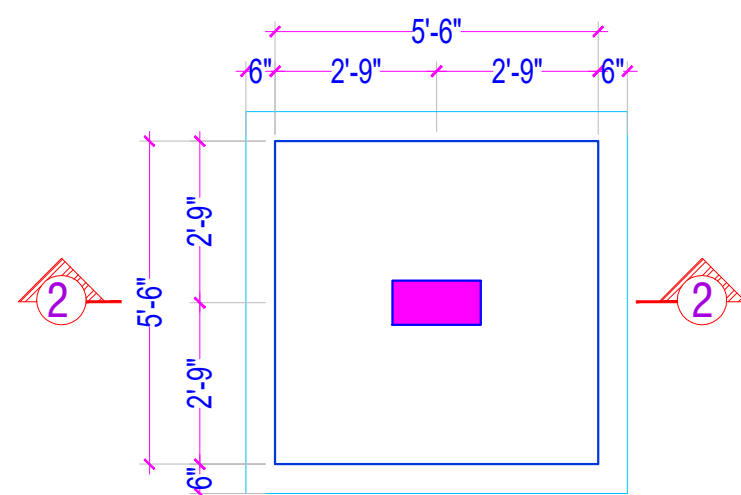
FOOTING F-2
