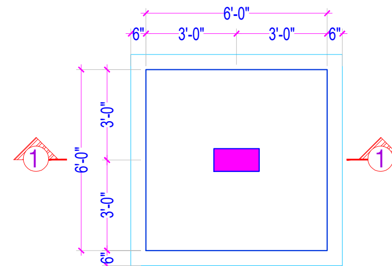
FOOTING F-1
