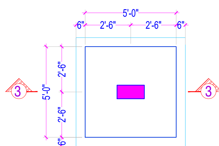
FOOTING F-3
