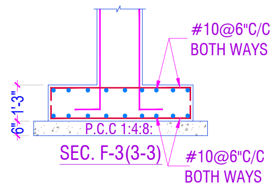
FOOTING F-3
