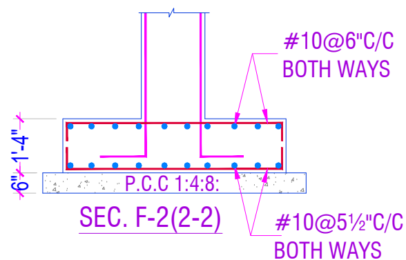
FOOTING F-2
