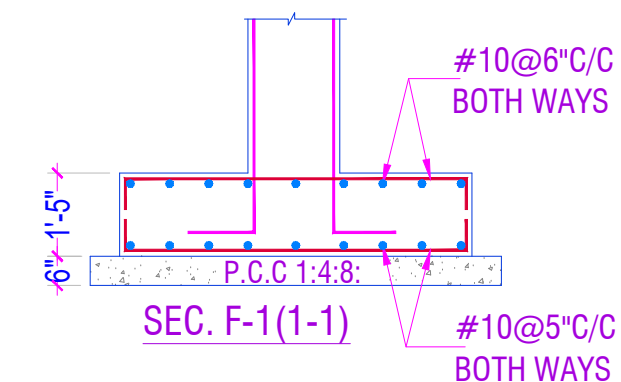
FOOTING F-1
