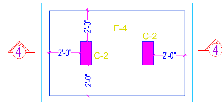
FOOTING F-4
