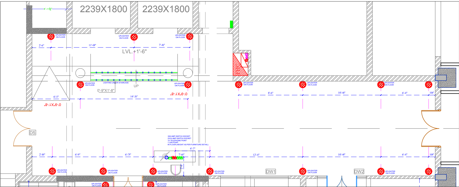
LOBBY REFLECTED FLOOR ELECTRICAL PLAN
