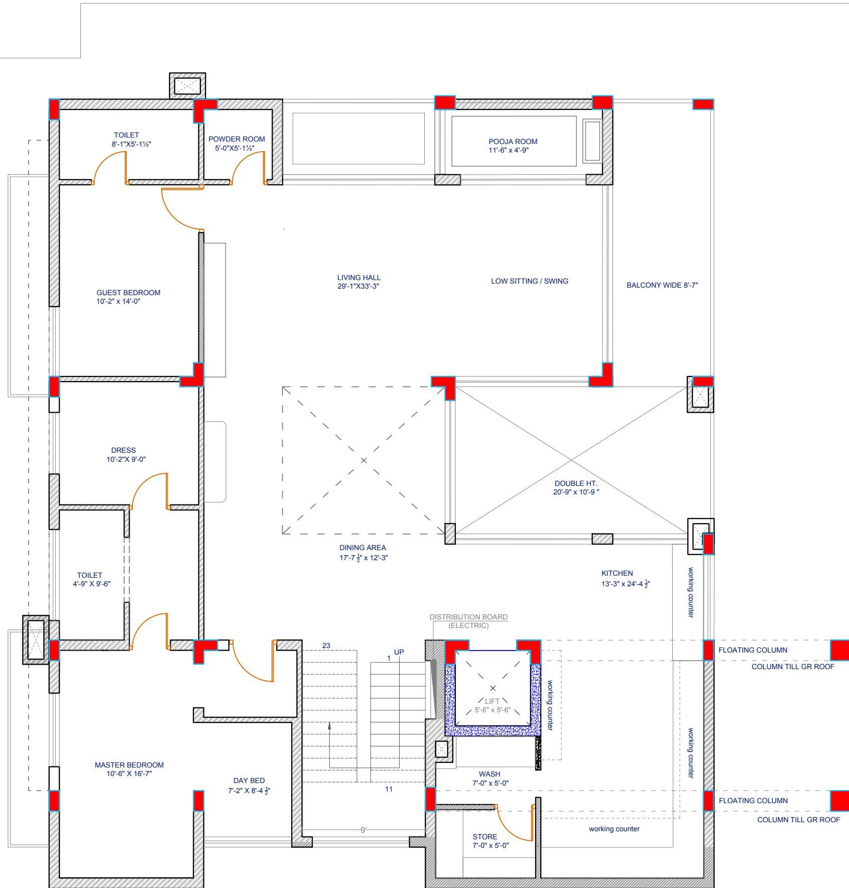
FIRST FLOOR
