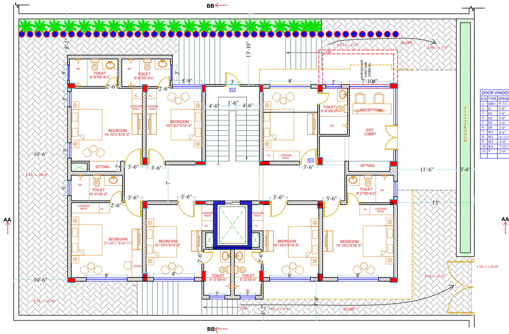
GROUND FLOOR
