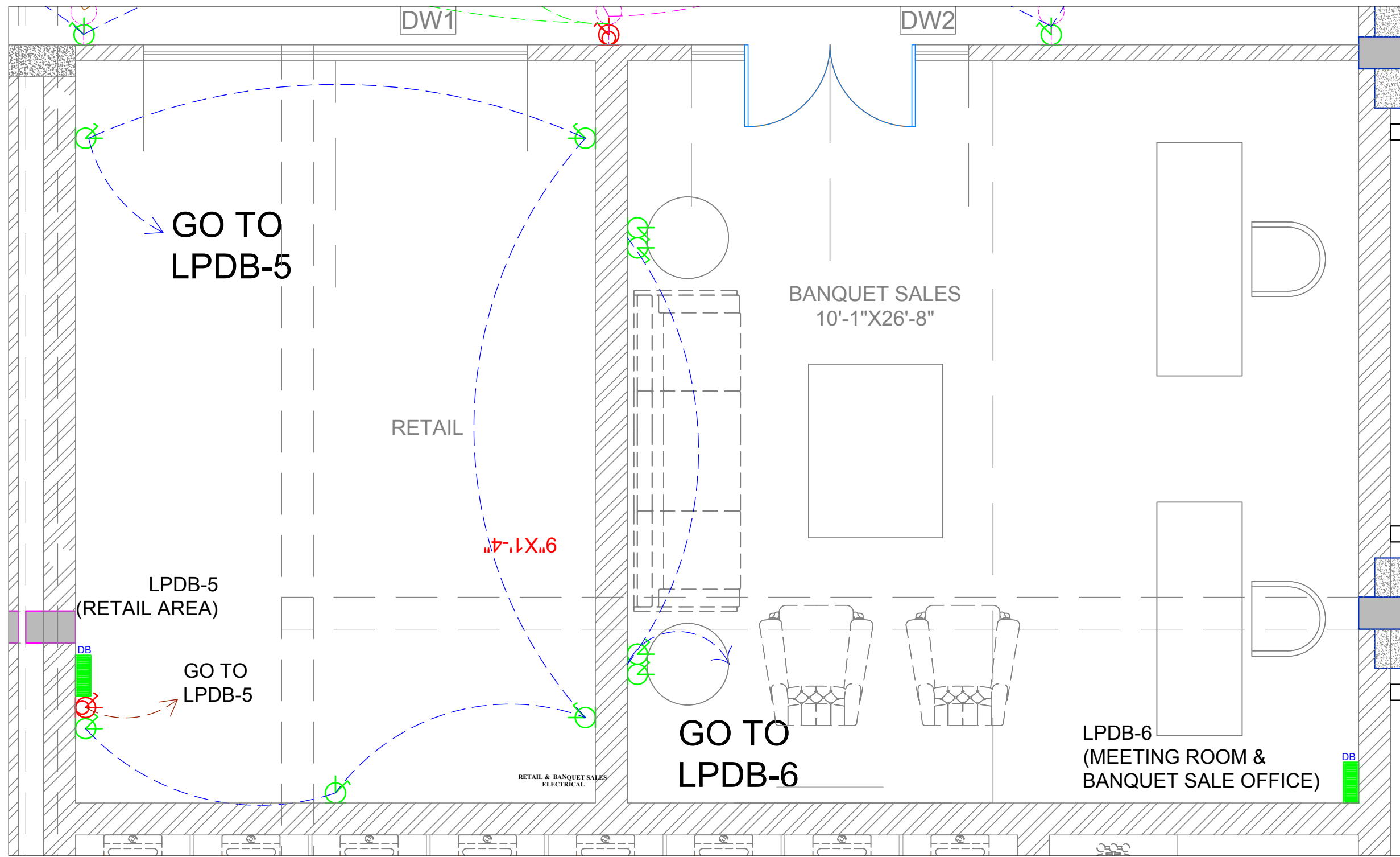
RETAIL & BANQUET SALES WALL WIRE DIAGRAM
