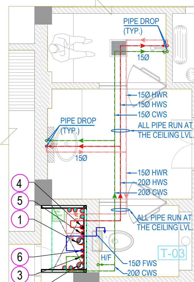
TOILET-03 FOR GROUND FLOOR (WATER SUPPLY LAYOUT)
