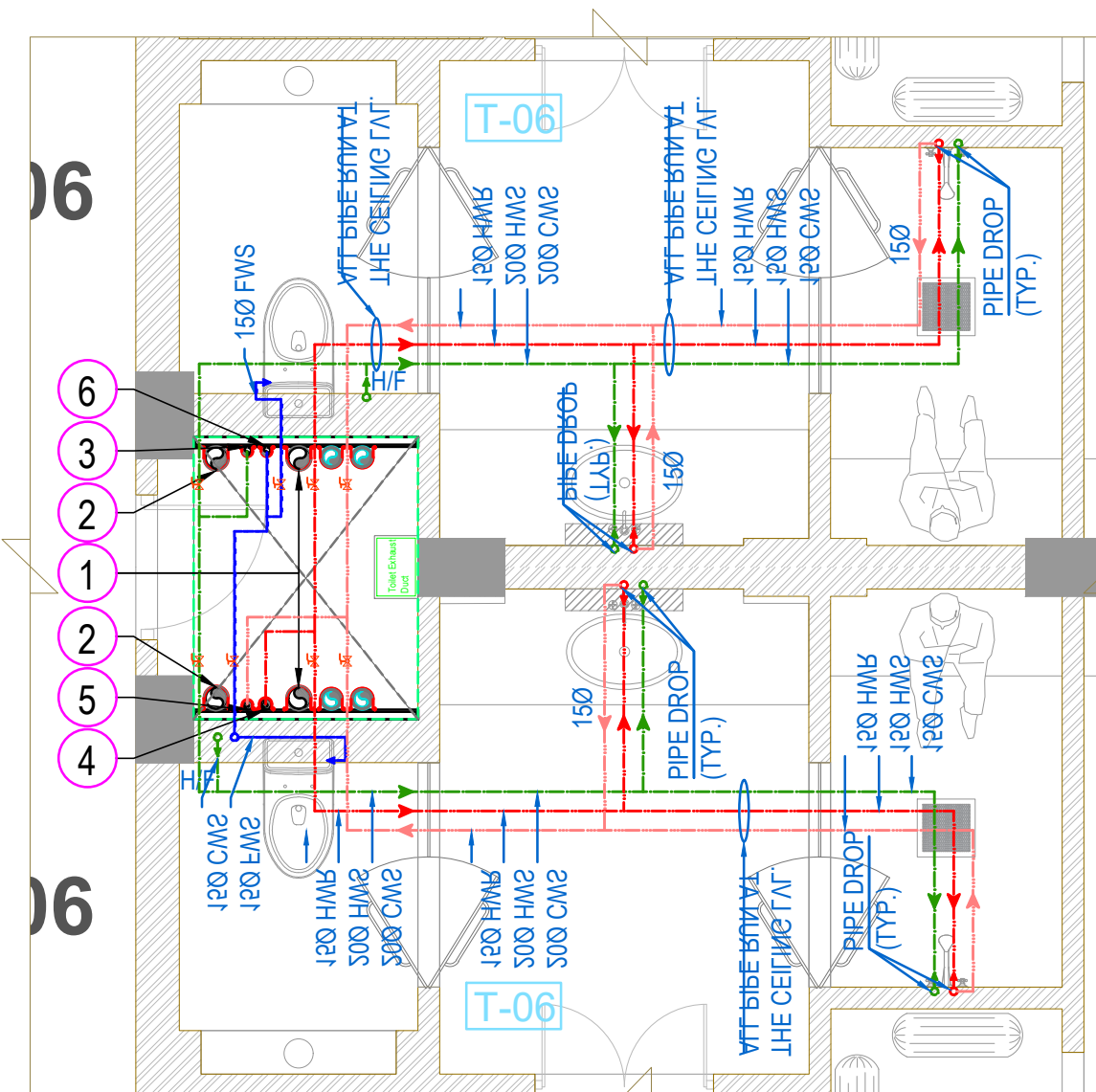
TOILET-06 FOR GROUND FLOOR (WATER SUPPLY LAYOUT)
