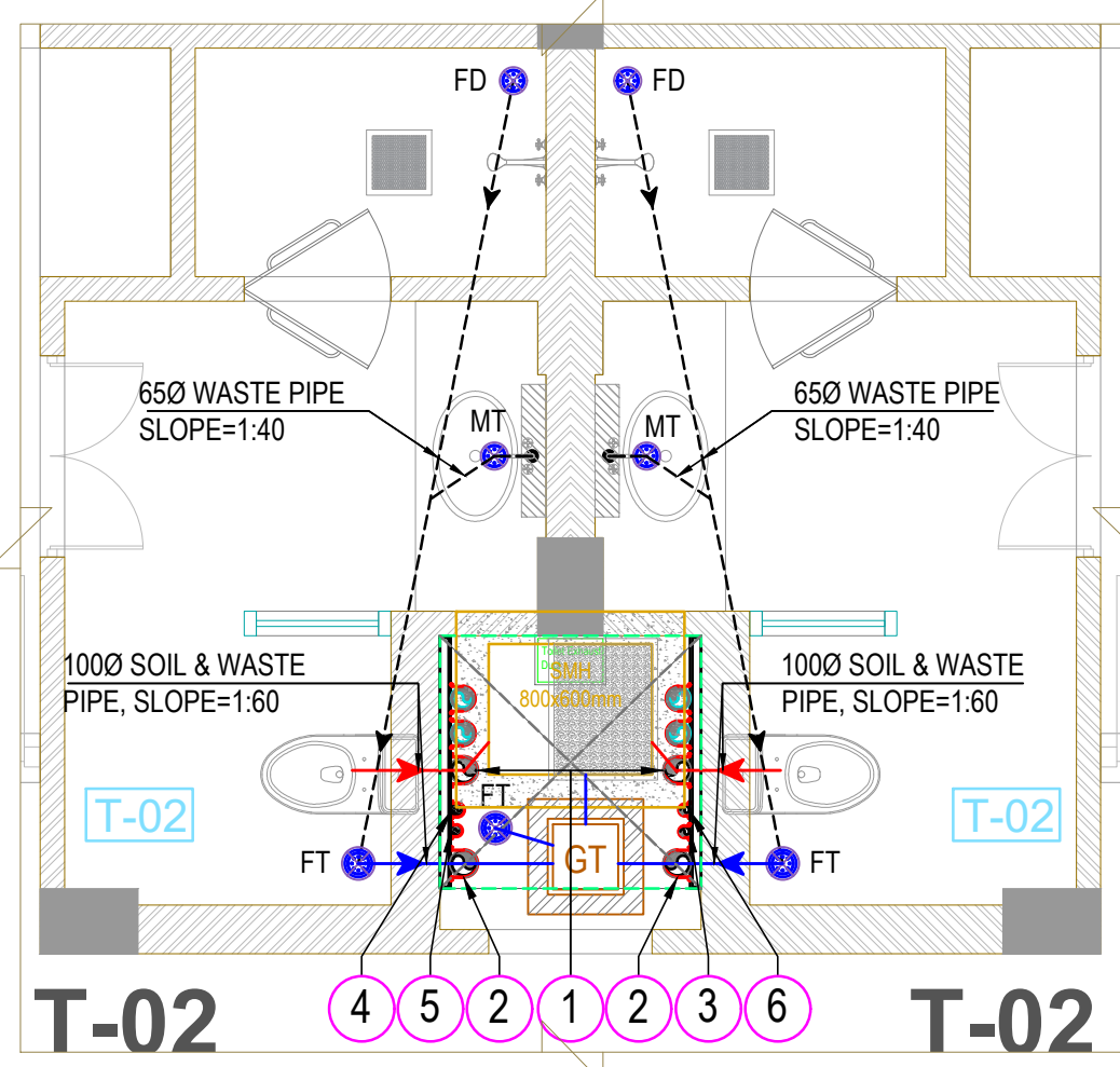
TOILET-02 FOR GROUND FLOOR (DRAINAGE LAYOUT)
