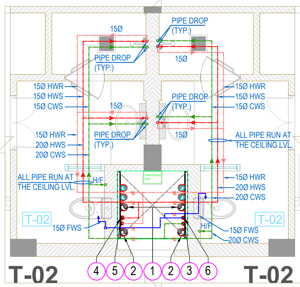
TOILET-02 FOR GROUND FLOOR (WATER SUPPLY LAYOUT)
