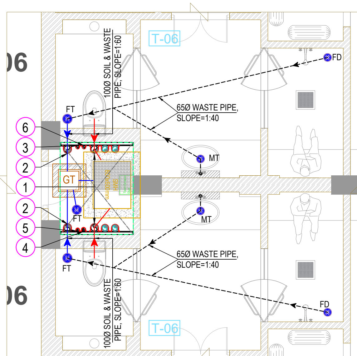
TOILET-06 FOR GROUND FLOOR (DRAINAGE LAYOUT)
