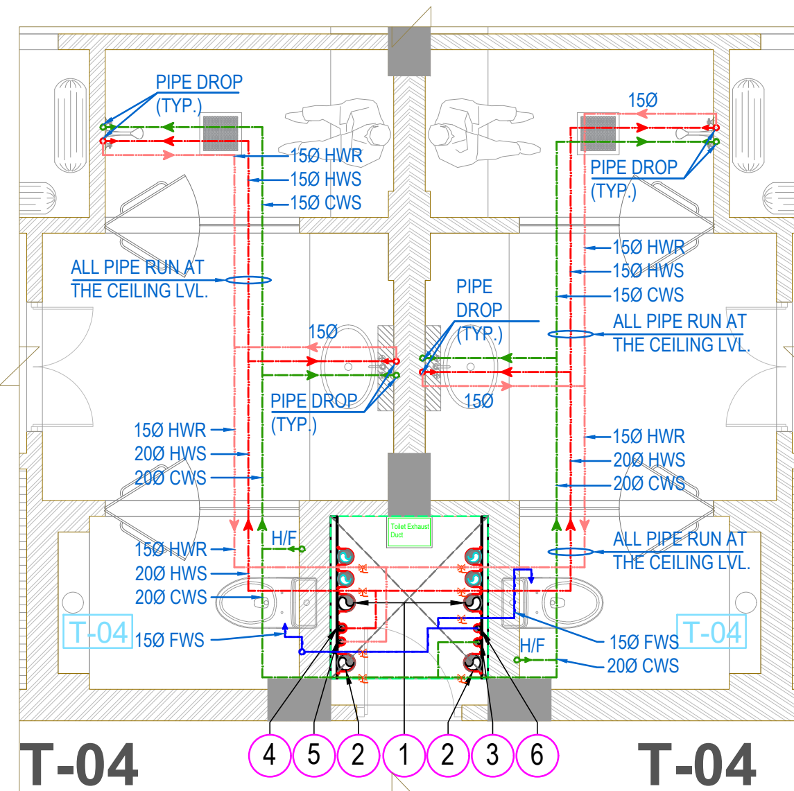
TOILET-04 FOR GROUND FLOOR (WATER SUPPLY LAYOUT)
