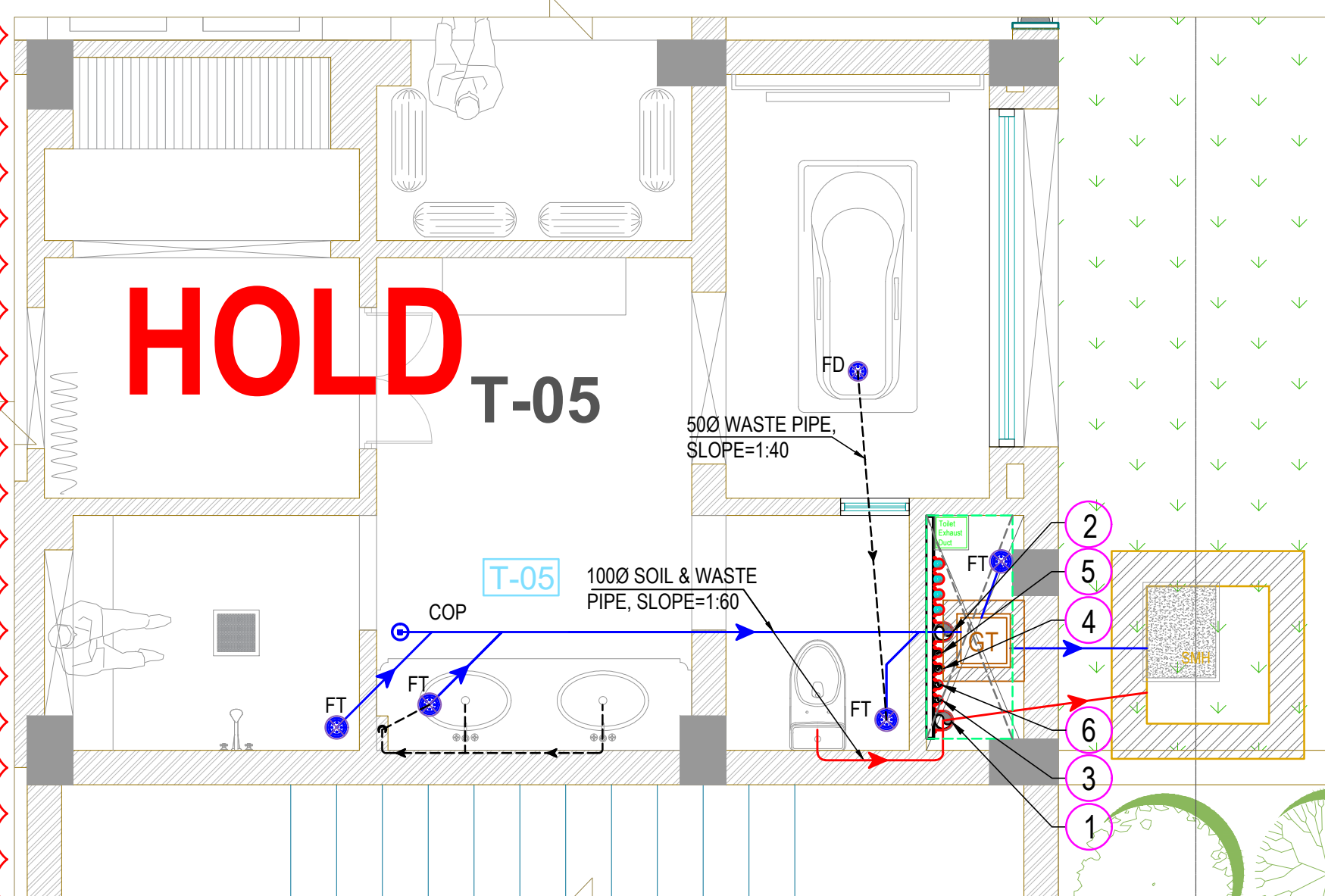
TOILET-05 FOR GROUND FLOOR (DRAINAGE LAYOUT)
