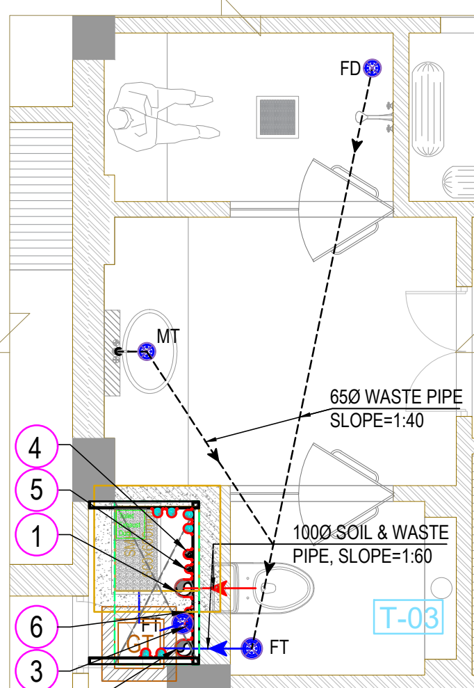
TOILET-03 FOR GROUND FLOOR (DRAINAGE LAYOUT)
