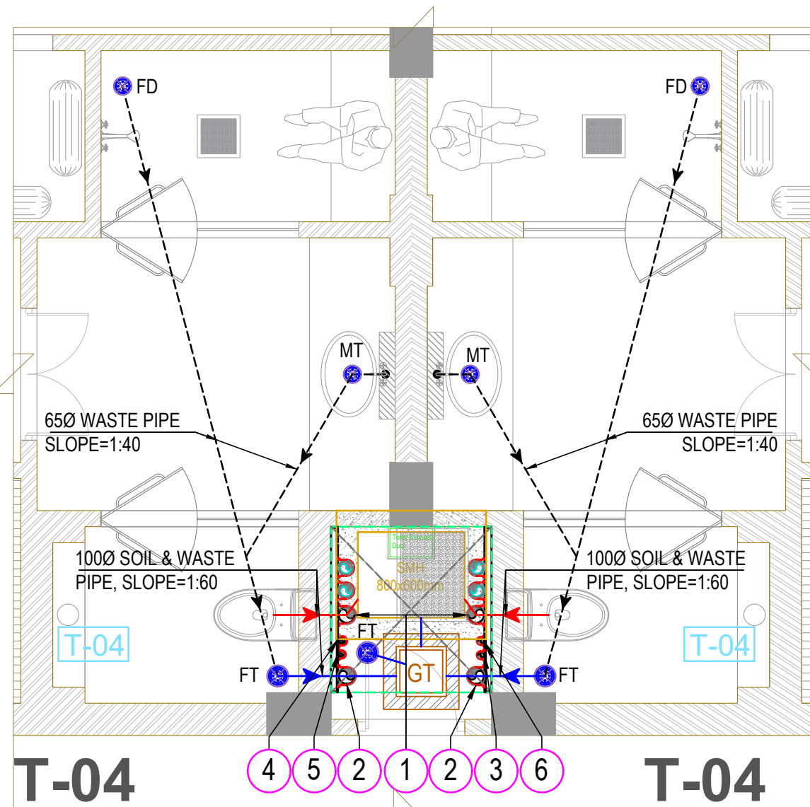
TOILET-04 FOR GROUND FLOOR (DRAINAGE LAYOUT)
