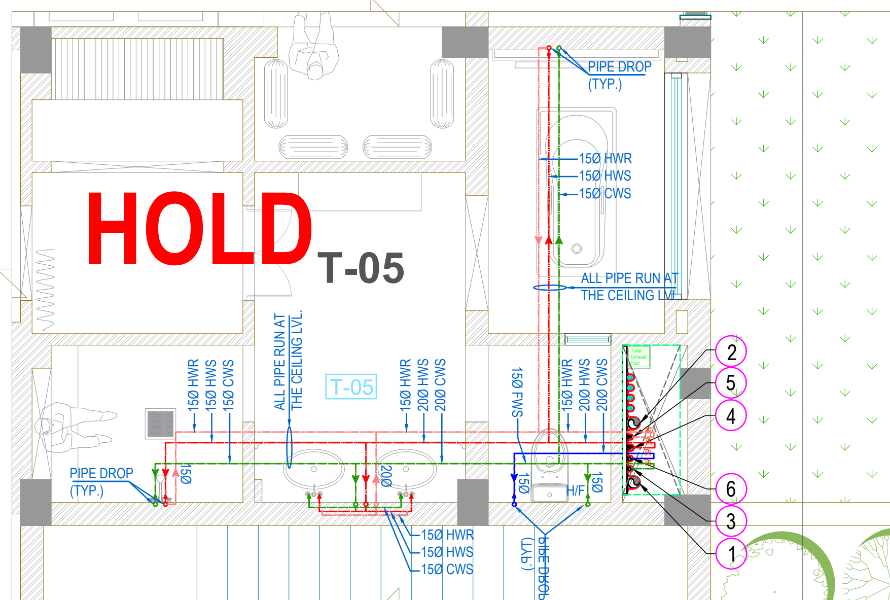
TOILET-05 FOR GROUND FLOOR (WATER SUPPLY LAYOUT)
