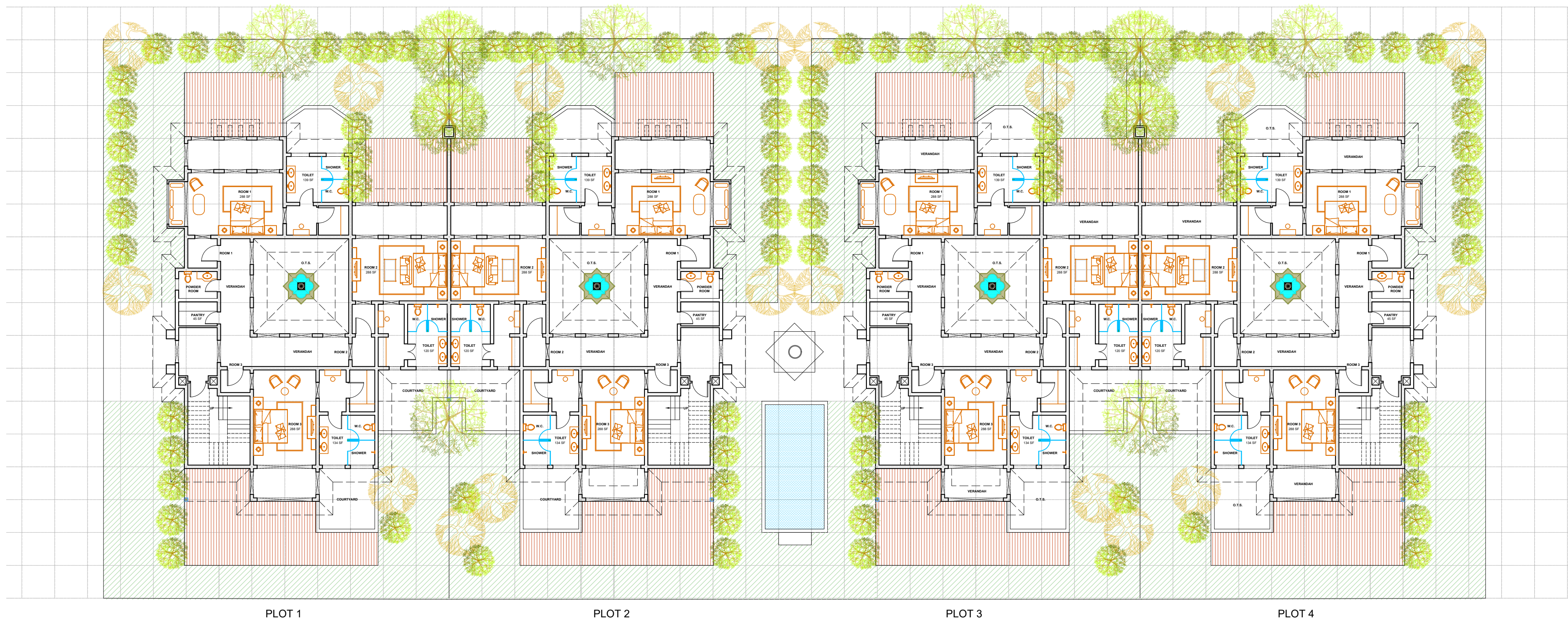
6 ROOM VILLA 1ST FLOOR PLAN
