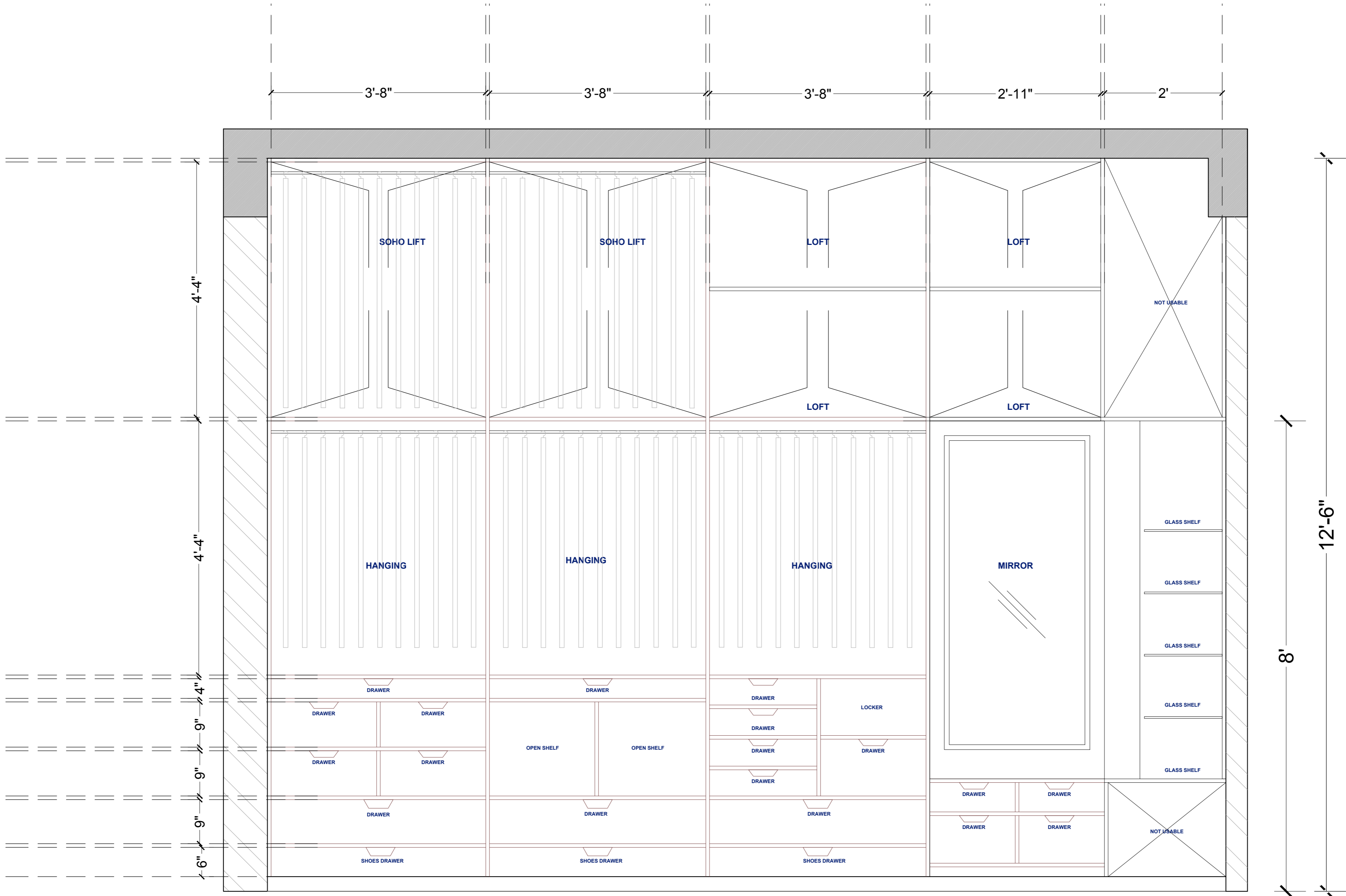
WARDROBE ELEVATION A
