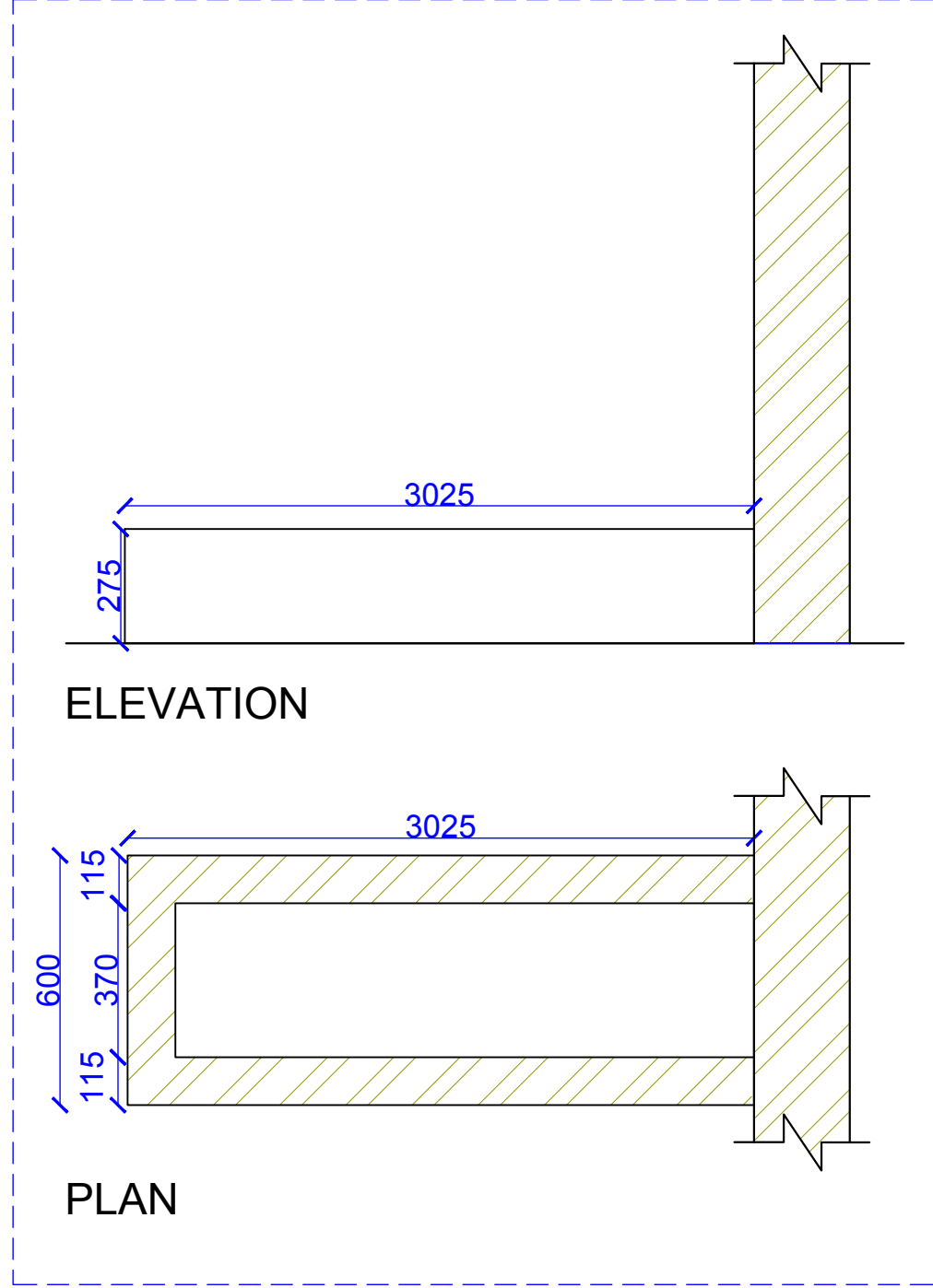
DETAIL A
