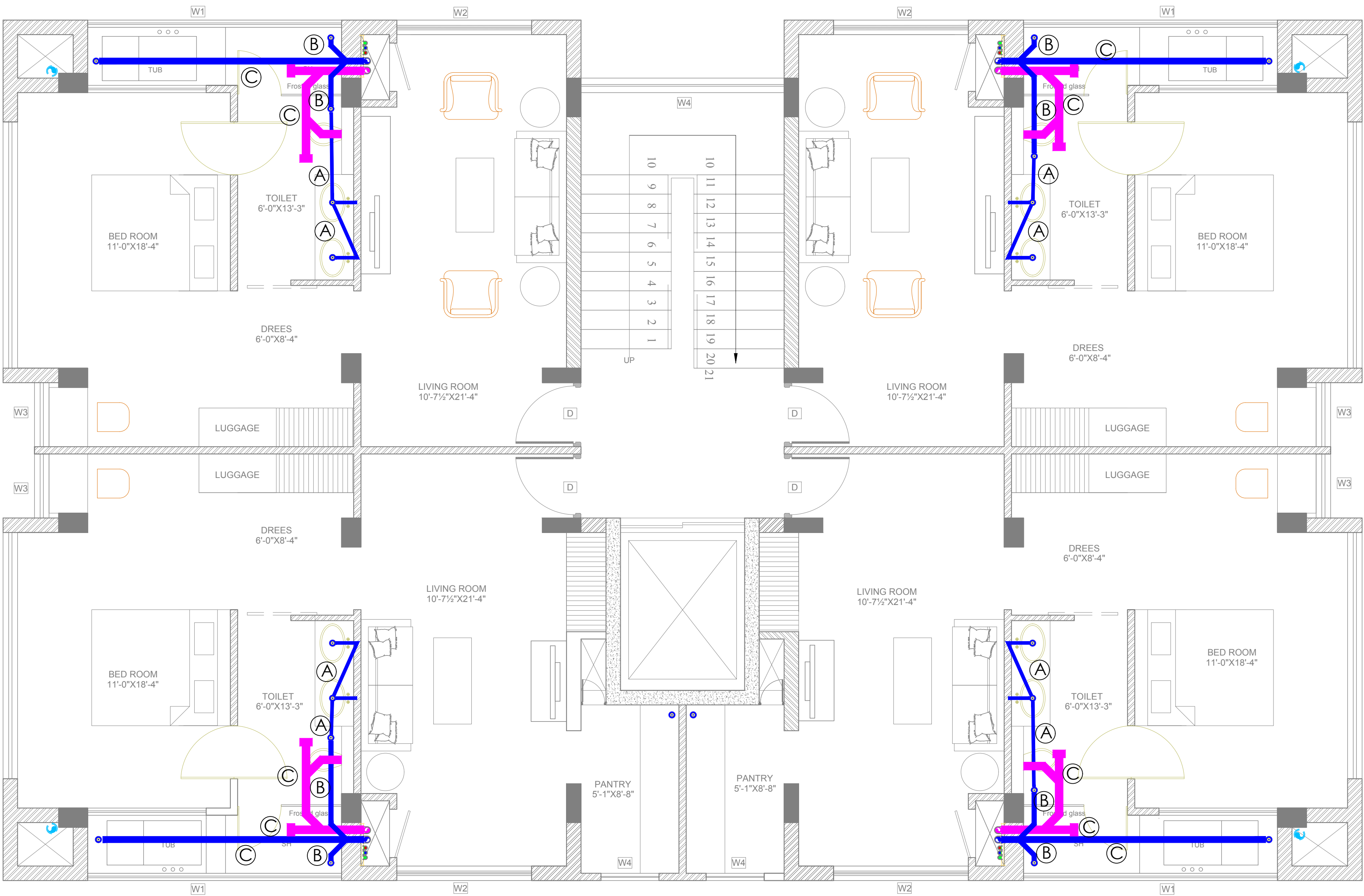
(R-12)-REVISED TYPICAL FLOOR PLAN DATE-22-12-2018
