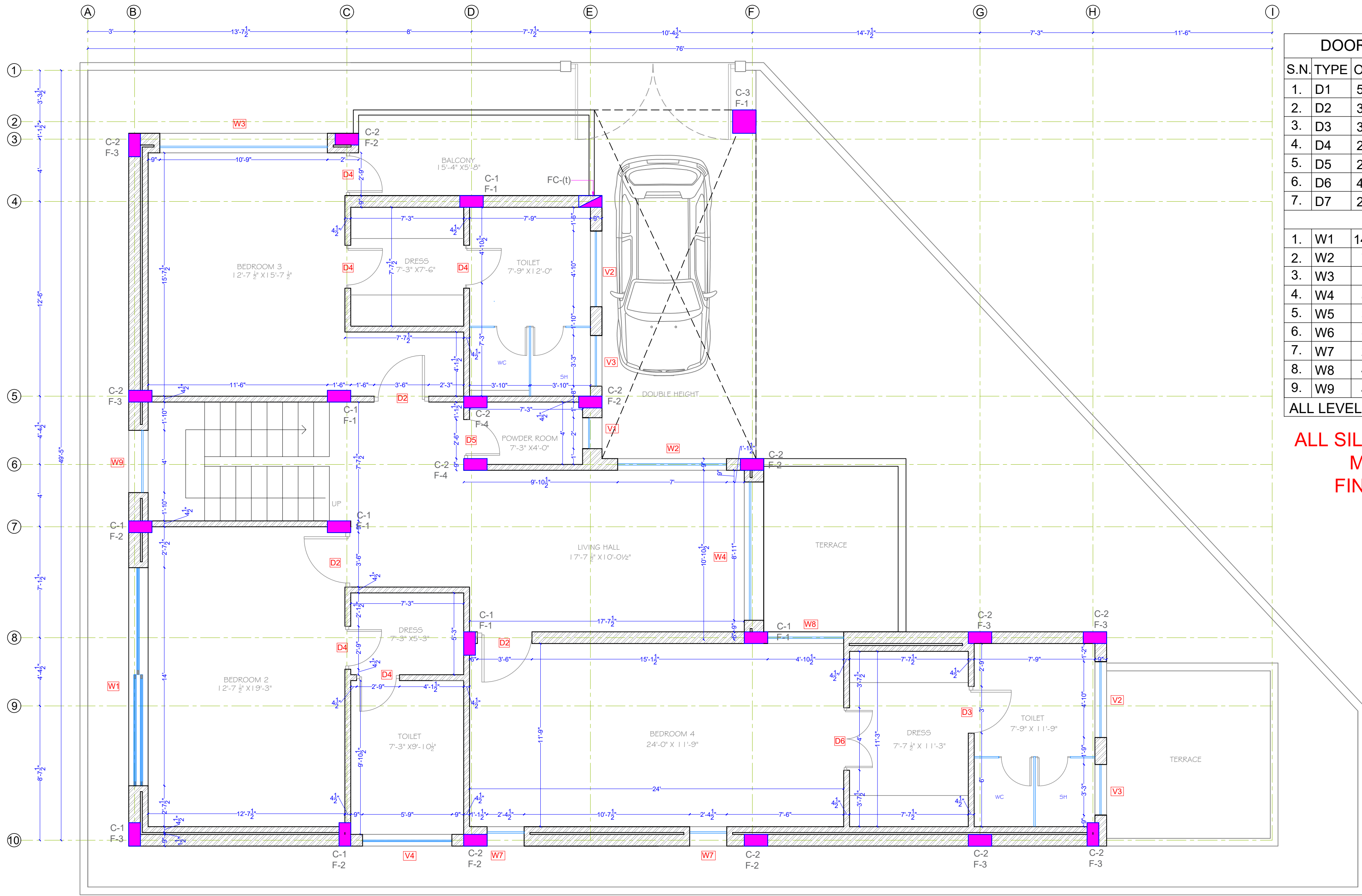
FIRST FLOOR
