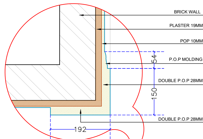
DETAIL-DD
