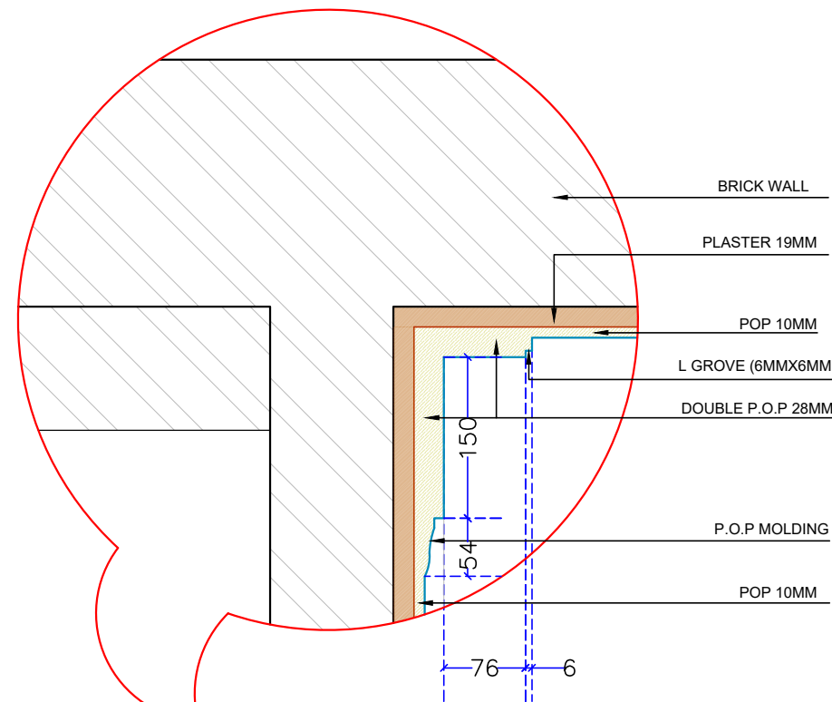
DETAIL-CC
