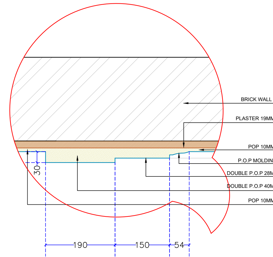
DETAIL-FF
