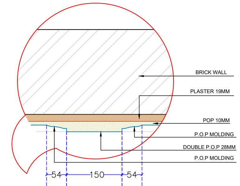
DETAIL-HH
