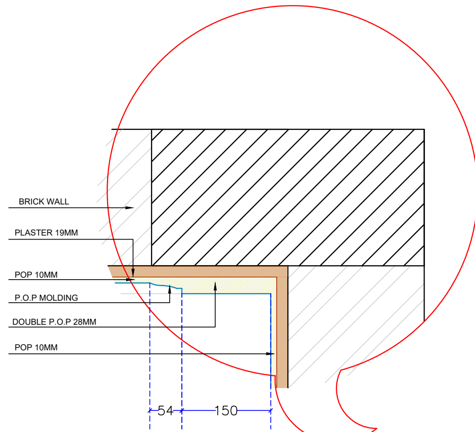
DETAIL-AA
