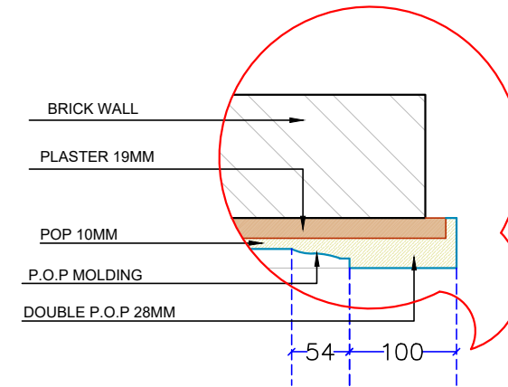
DETAIL-EE
