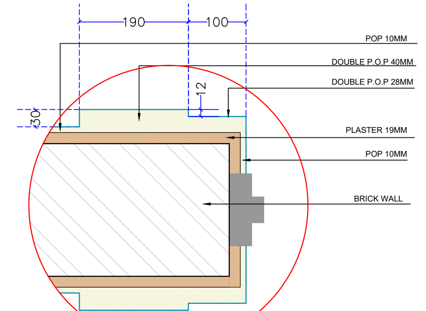
DETAIL FF
