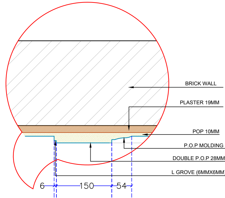
DETAIL-BB
