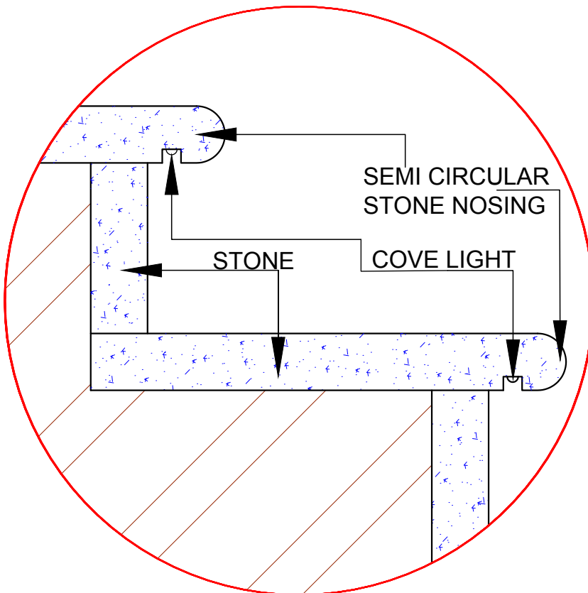
LIGHTING DETAIL FOR STAIRS AT BAVDI
