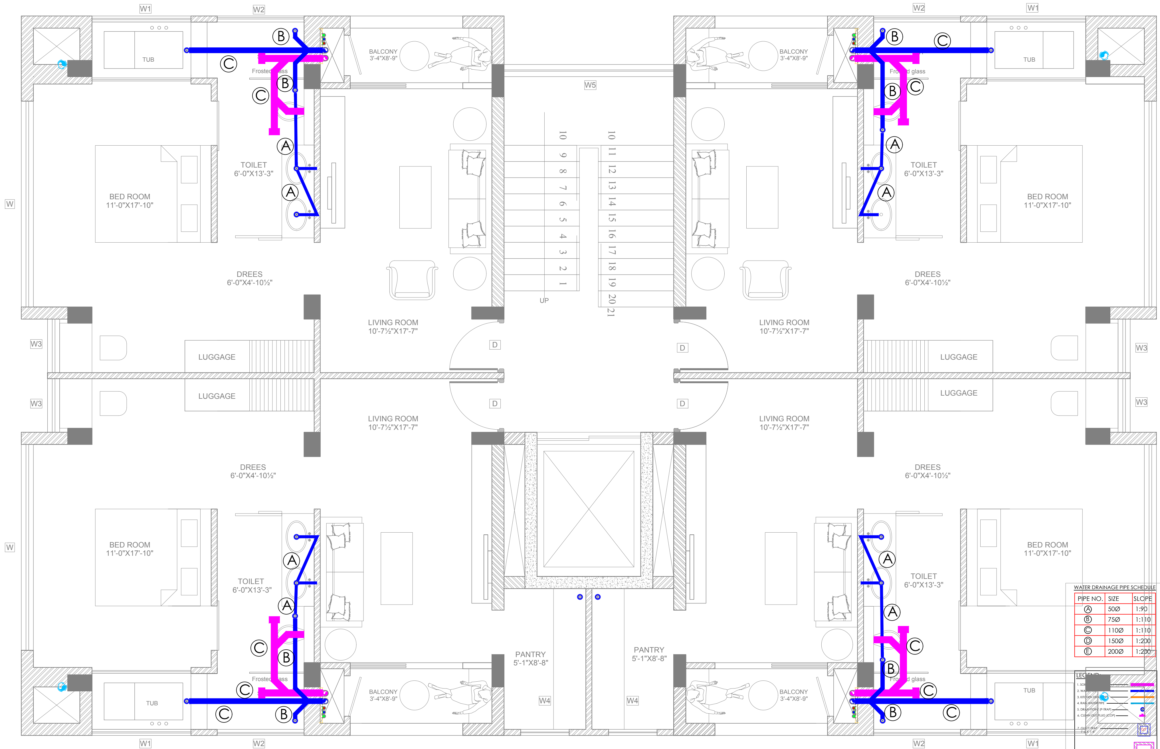
(R-11)-REVISED TYPICAL FLOOR PLAN
