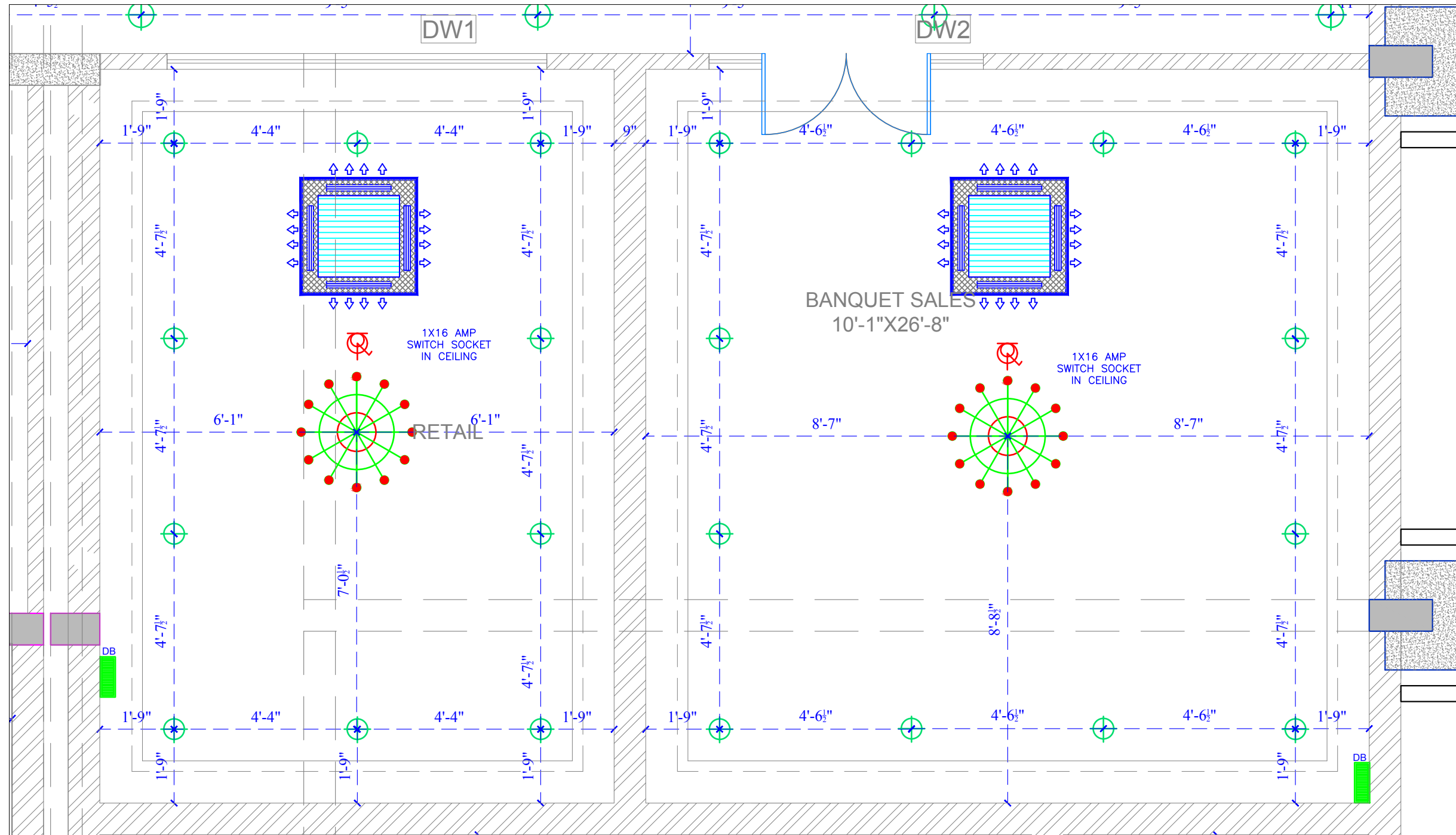
RETAIL & BANQUET SALES REFLECTED CEILING ELECTRICAL PLAN
