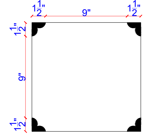
DETAIL 1
