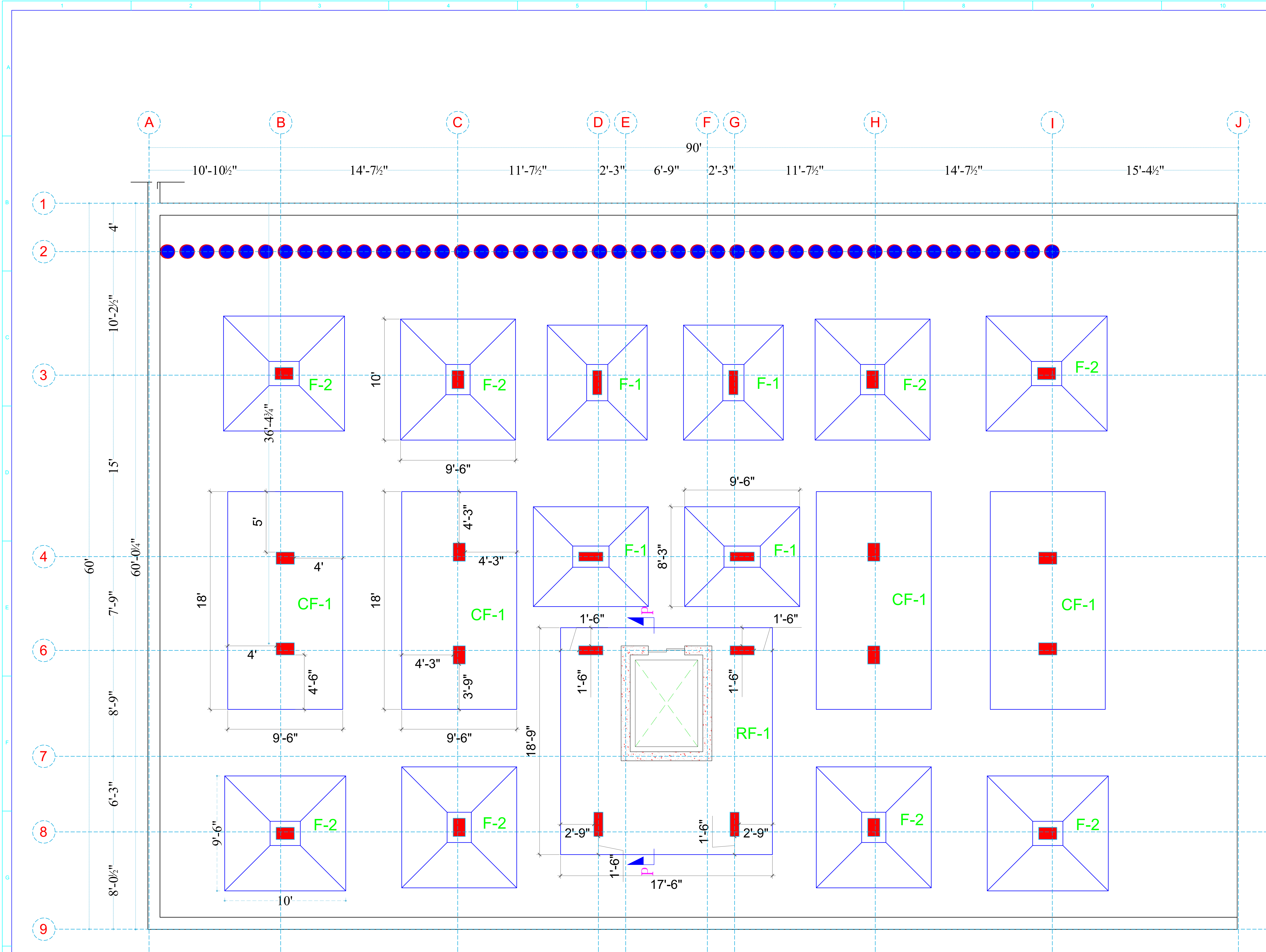
FOUNDATONN LAYOUT PLAN
