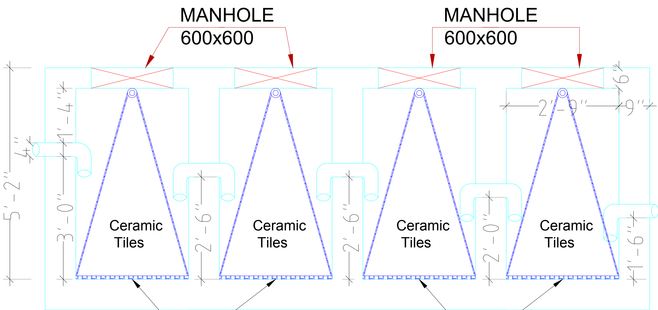
S.S. Perforated Tray
