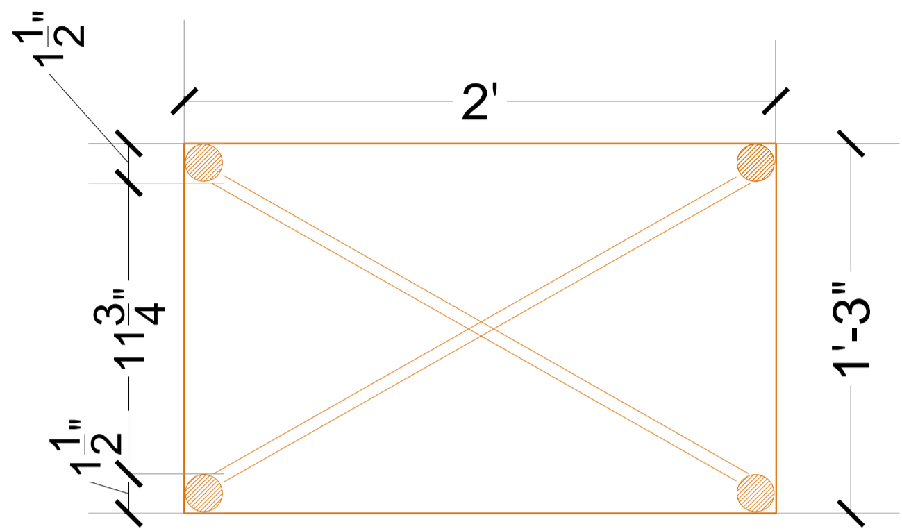
OTTOMAN PLAN
