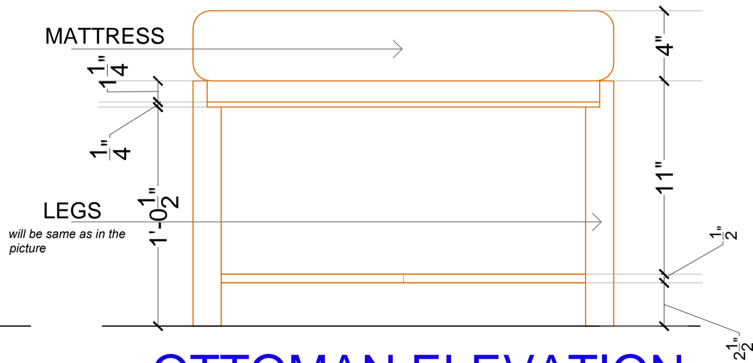
OTTOMAN ELEVATION
