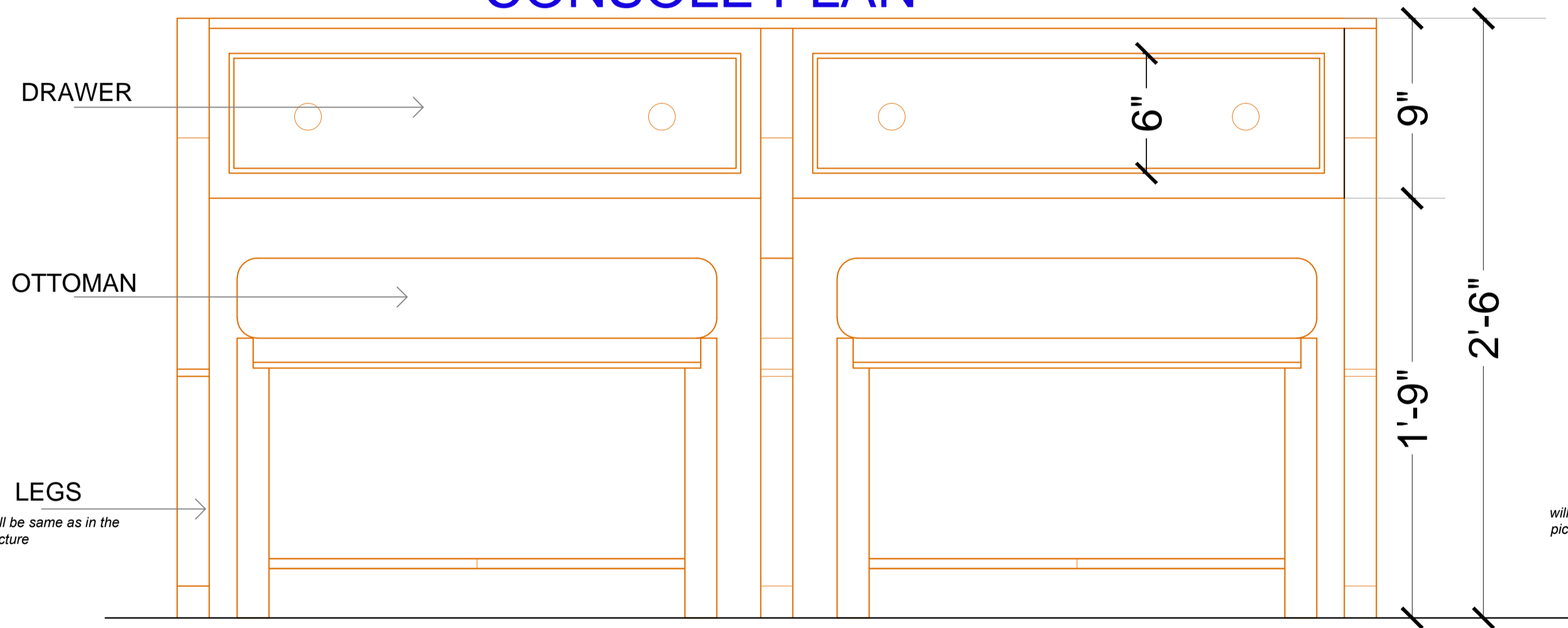
CONSOLE ELEVATION
