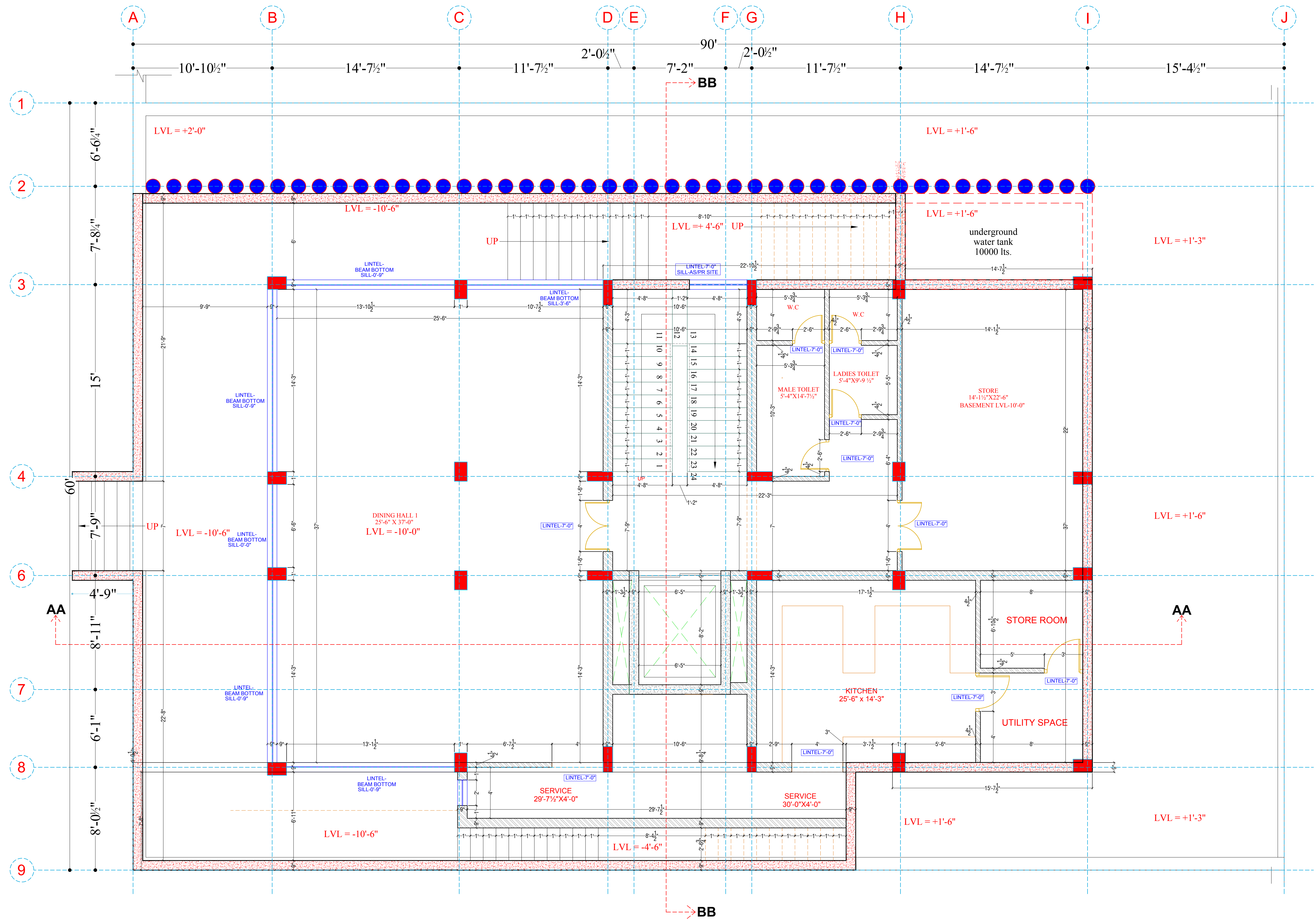
ALL LINTEL AND SILL LVL F.F FLOOR BASEMENT FLOOR WORKING DRAWING
