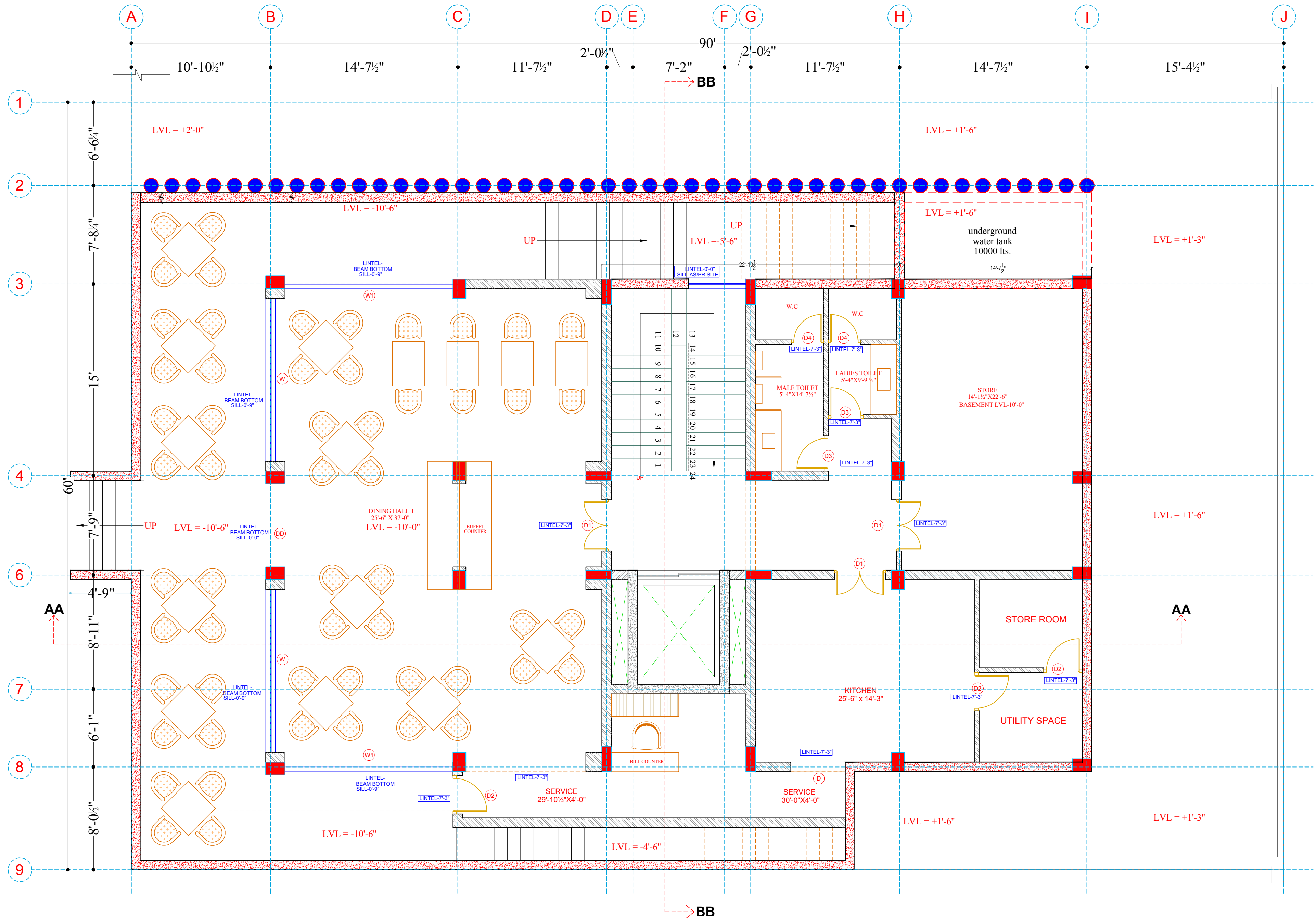
BASEMENT FLOOR DRAWING
