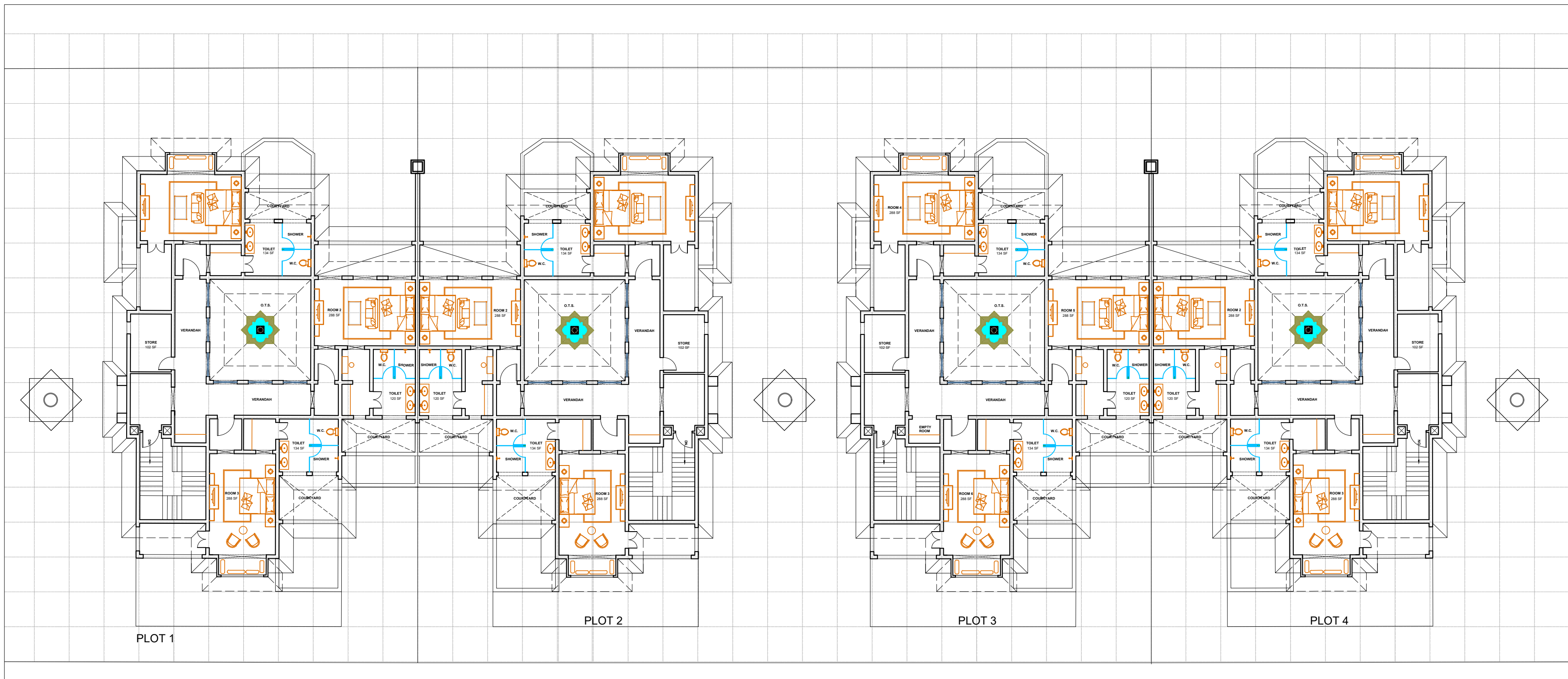
6 ROOM VILLA 1ST FLOOR PLAN
