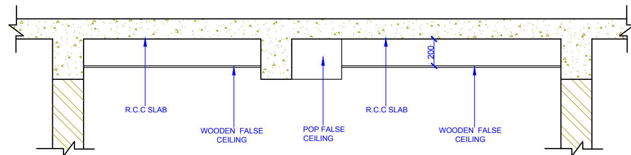
SECTION YY'
