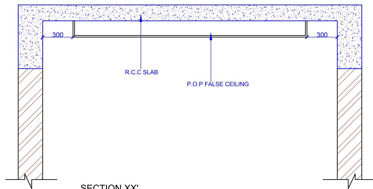
SECTION XX'
