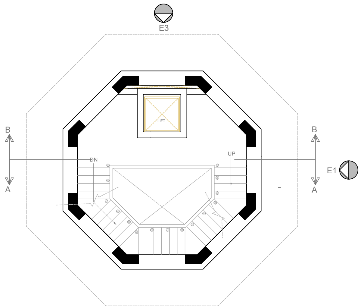
PLAN AT LEVEL +3.45M
