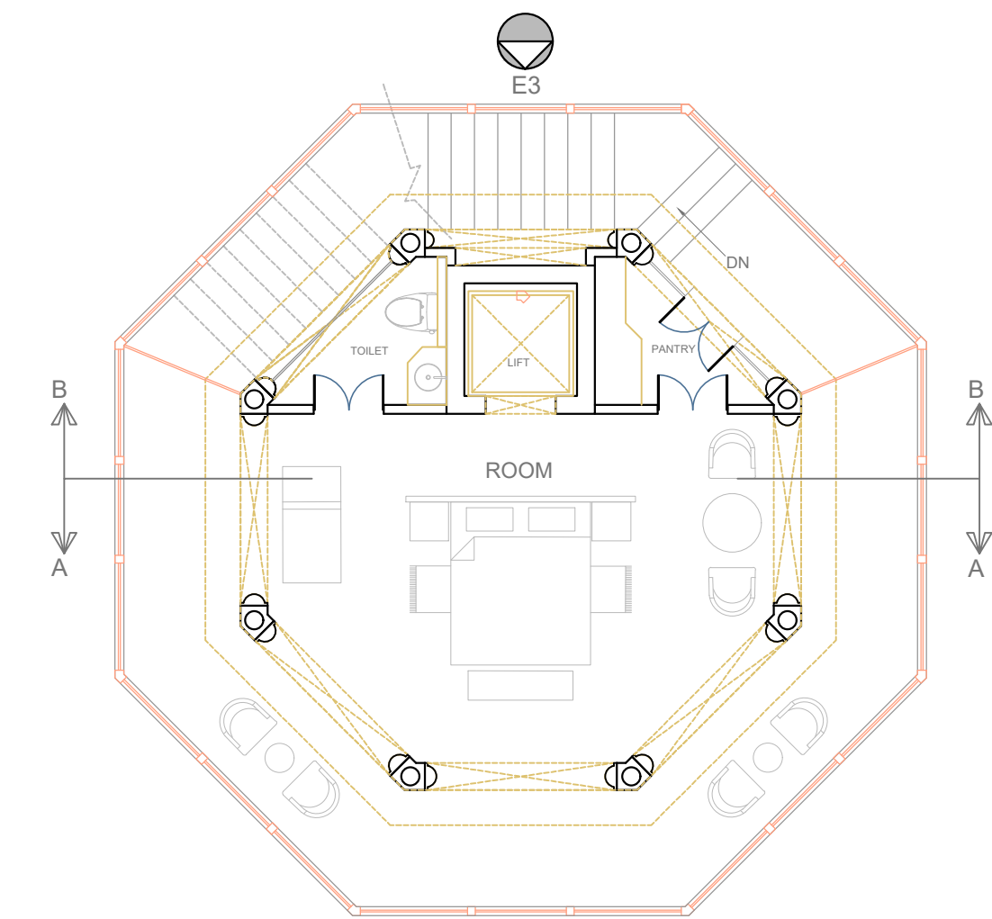
PLAN AT LEVEL +20.25M
