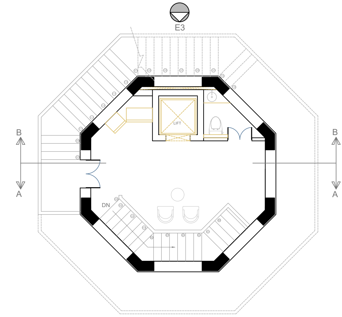
PLAN AT LEVEL +15.90M
