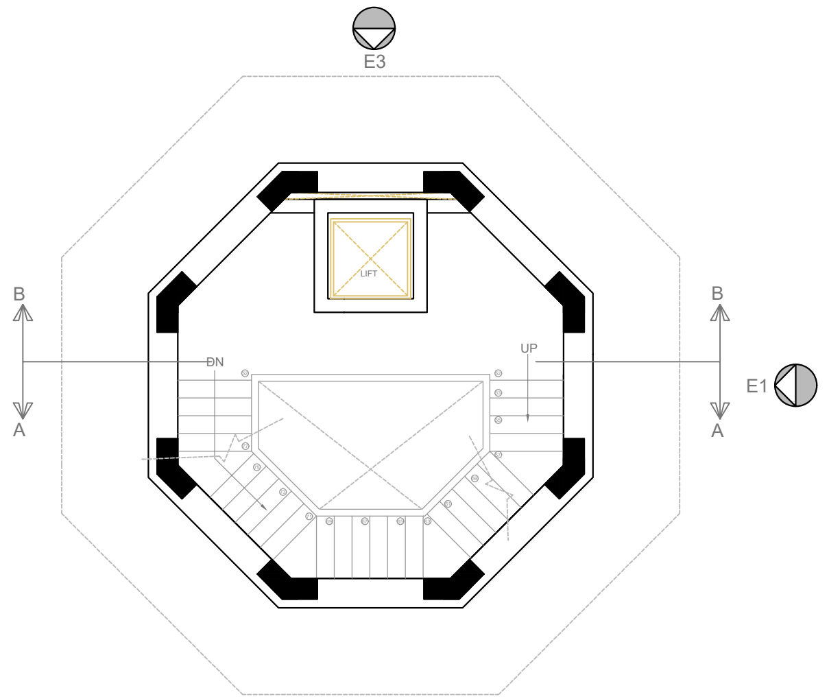
PLAN AT LEVEL +7.8M
