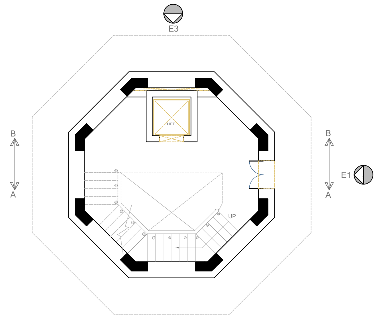
PLAN AT LEVEL +0.00M
