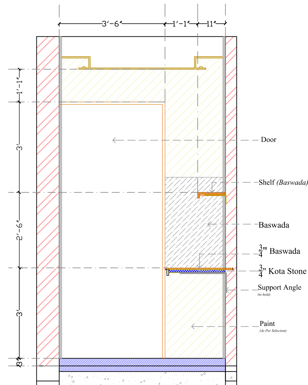
ELEVATION D
