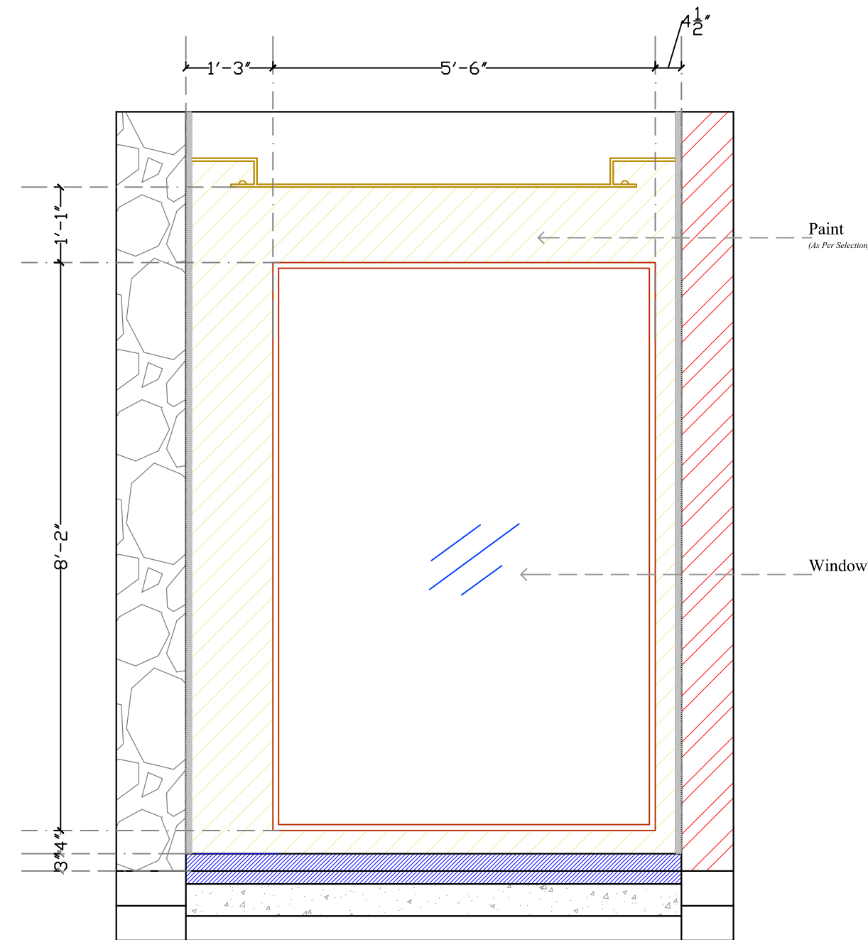
ELEVATION C
