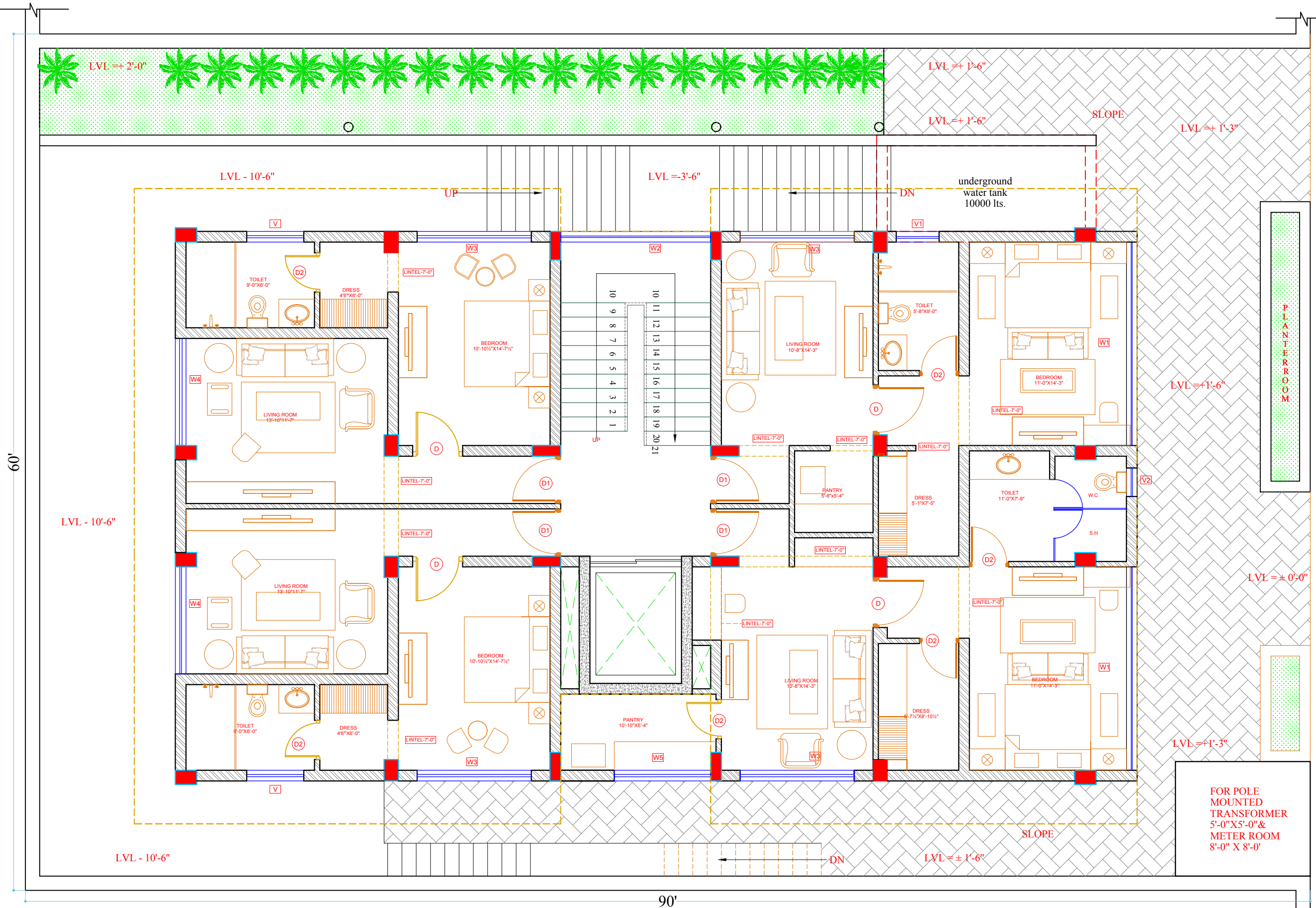
REVISED GROUND FLOOR
