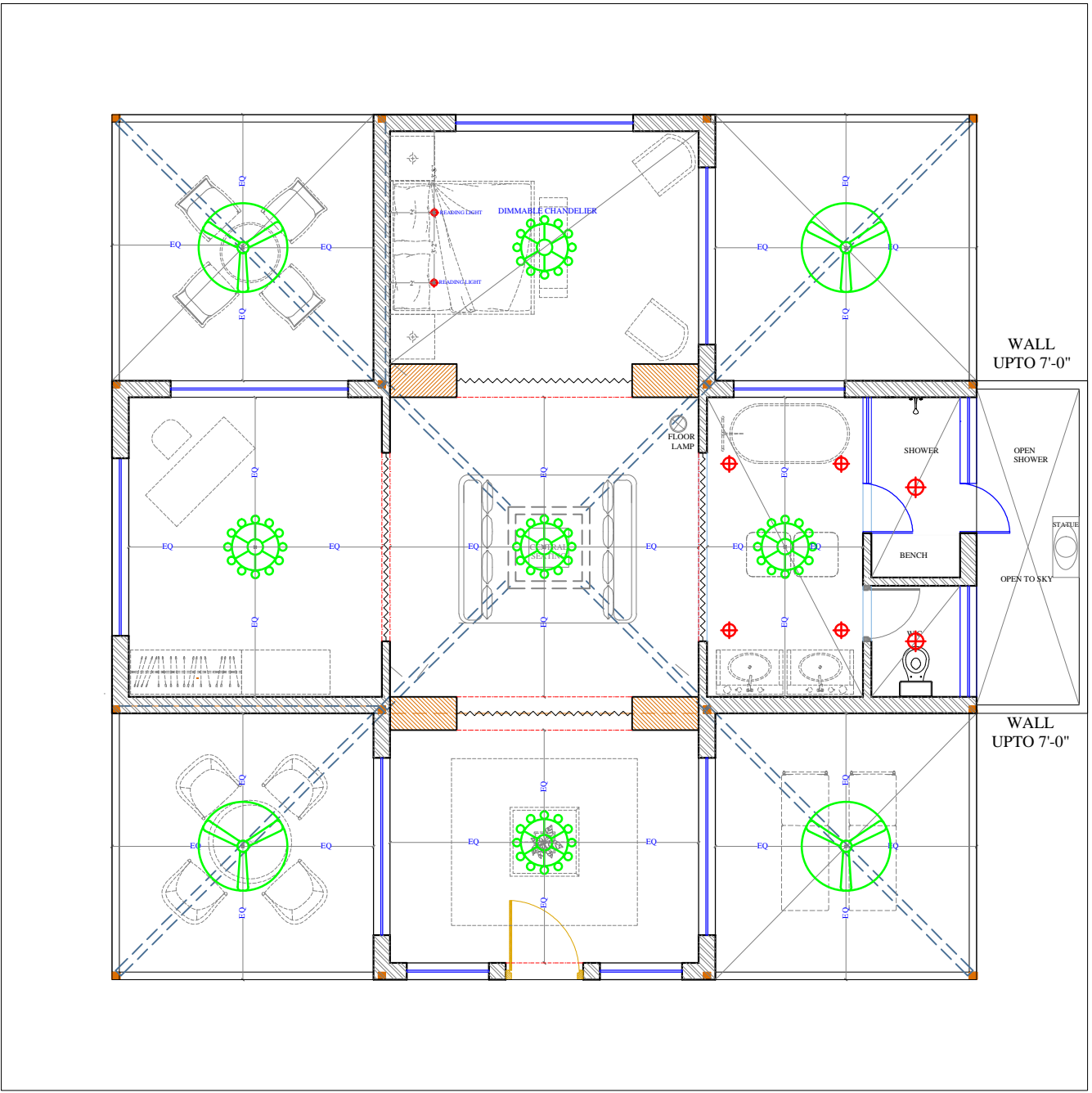
CEILING ELECTRICAL
