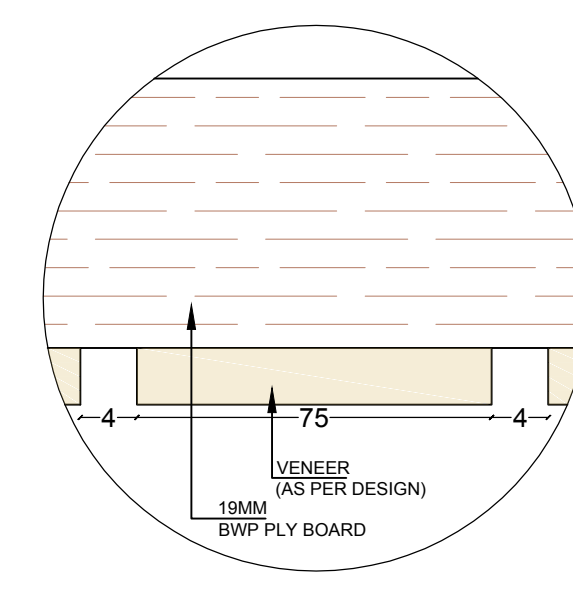
DETAIL AT X (SECTION)
