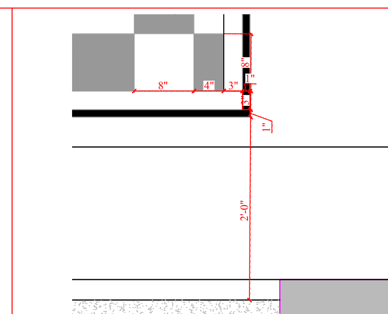
DETAIL AT FD9
