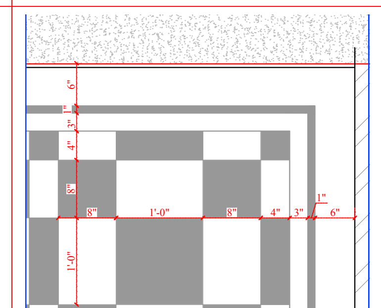
DETAIL AT FD12
