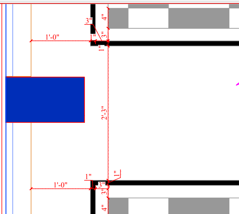
DETAIL AT FD2
