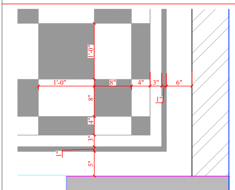
DETAIL AT FD10
