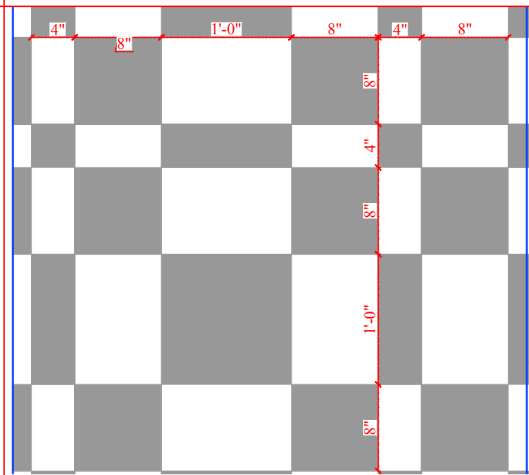
DETAIL AT FD4
