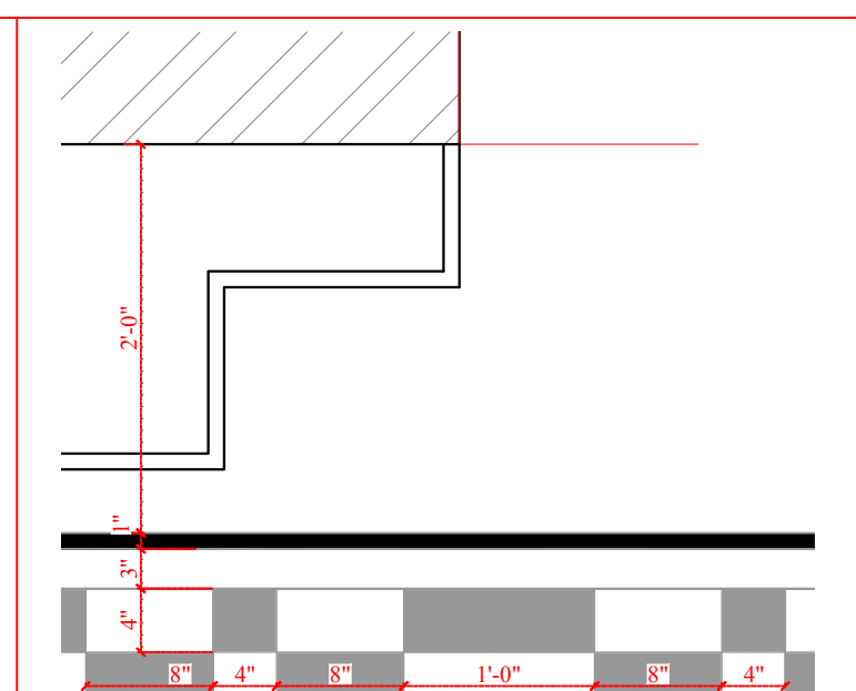
DETAIL AT FD8
