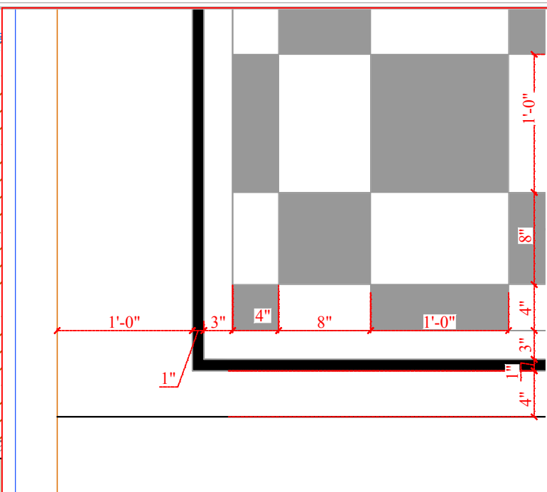
DETAIL AT FD1
