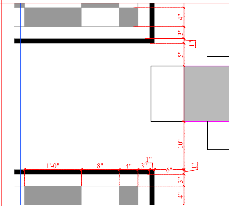
DETAIL AT FD6
