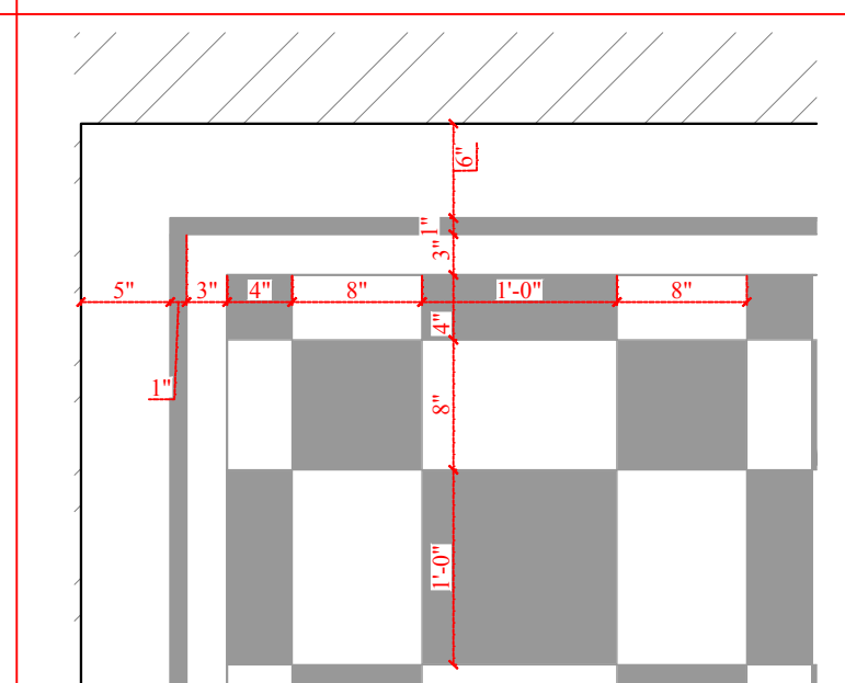
DETAIL AT FD11
