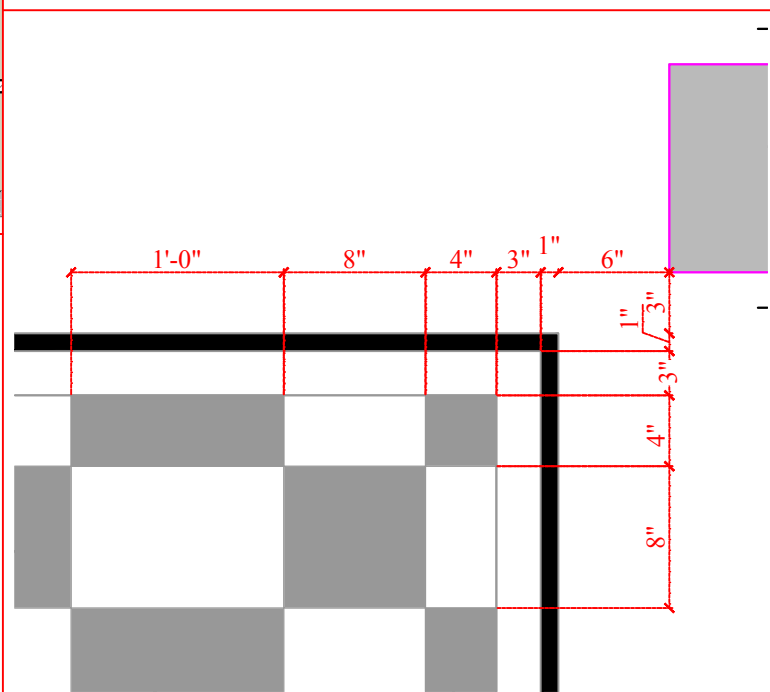
DETAIL AT FD5
