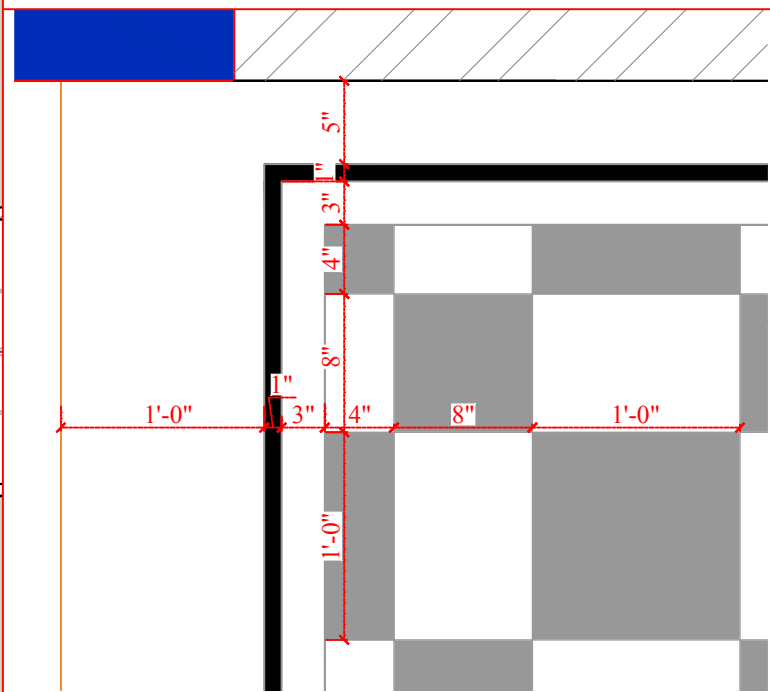
DETAIL AT FD3
