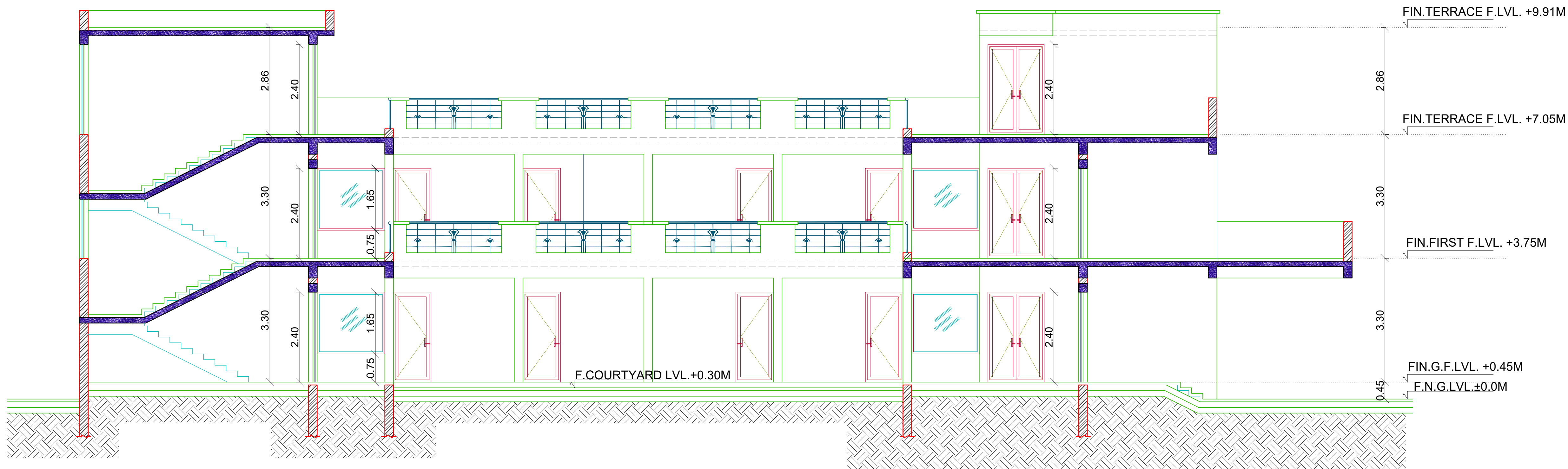
SECTION X-X
