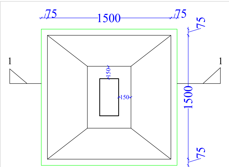
FOUNDATION (F1)
