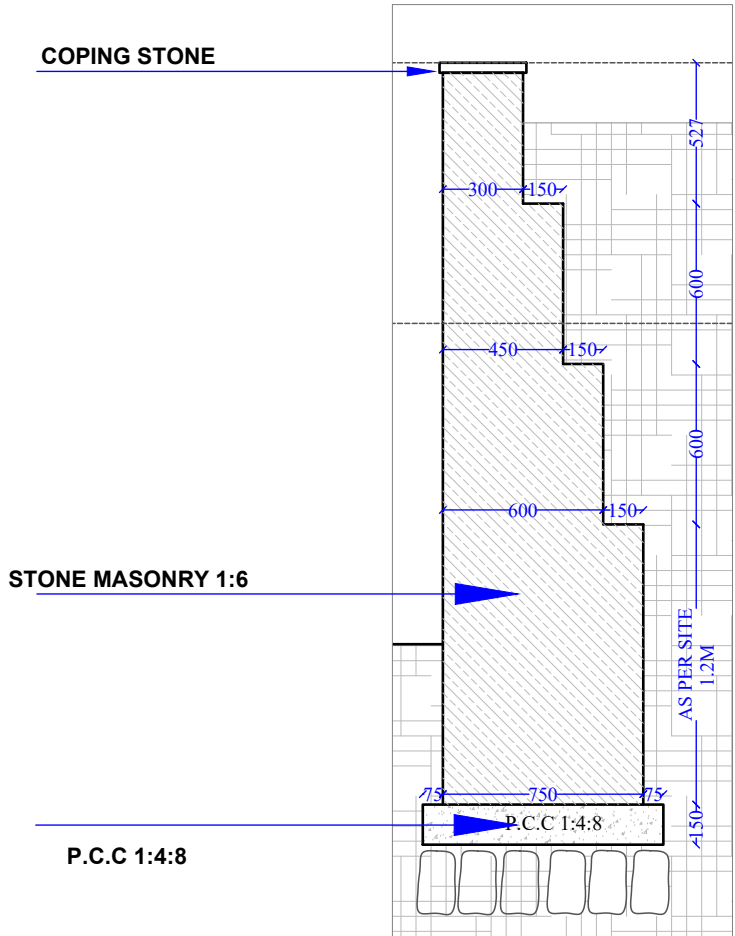
TYPICAL WALL SECTION (OUTER)
