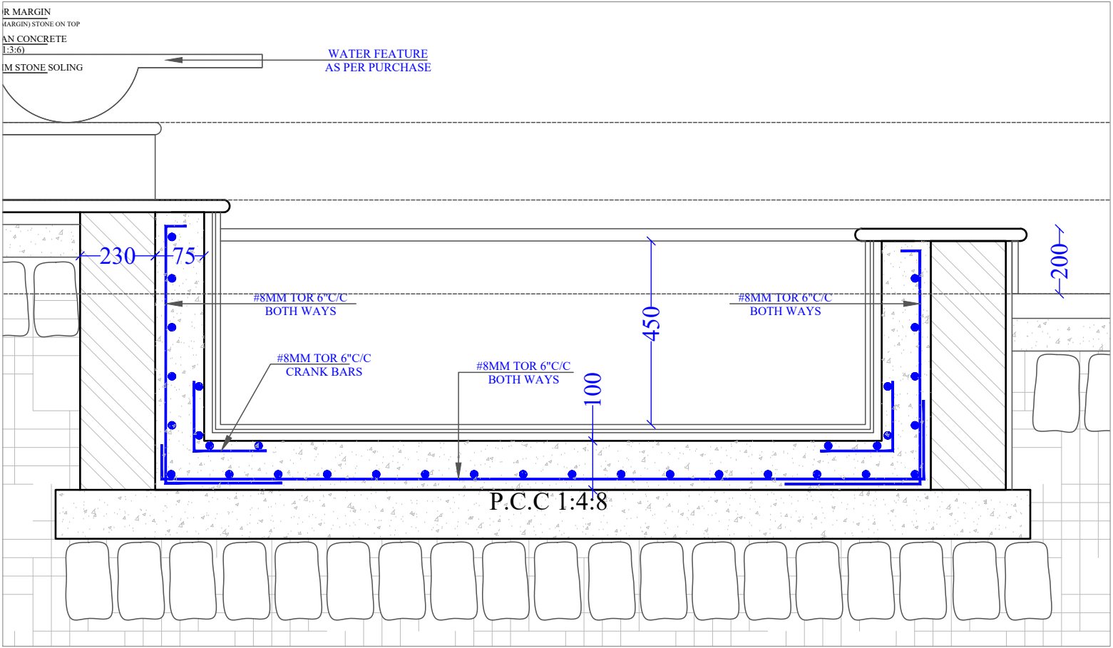
WATER BODY DETAIL
