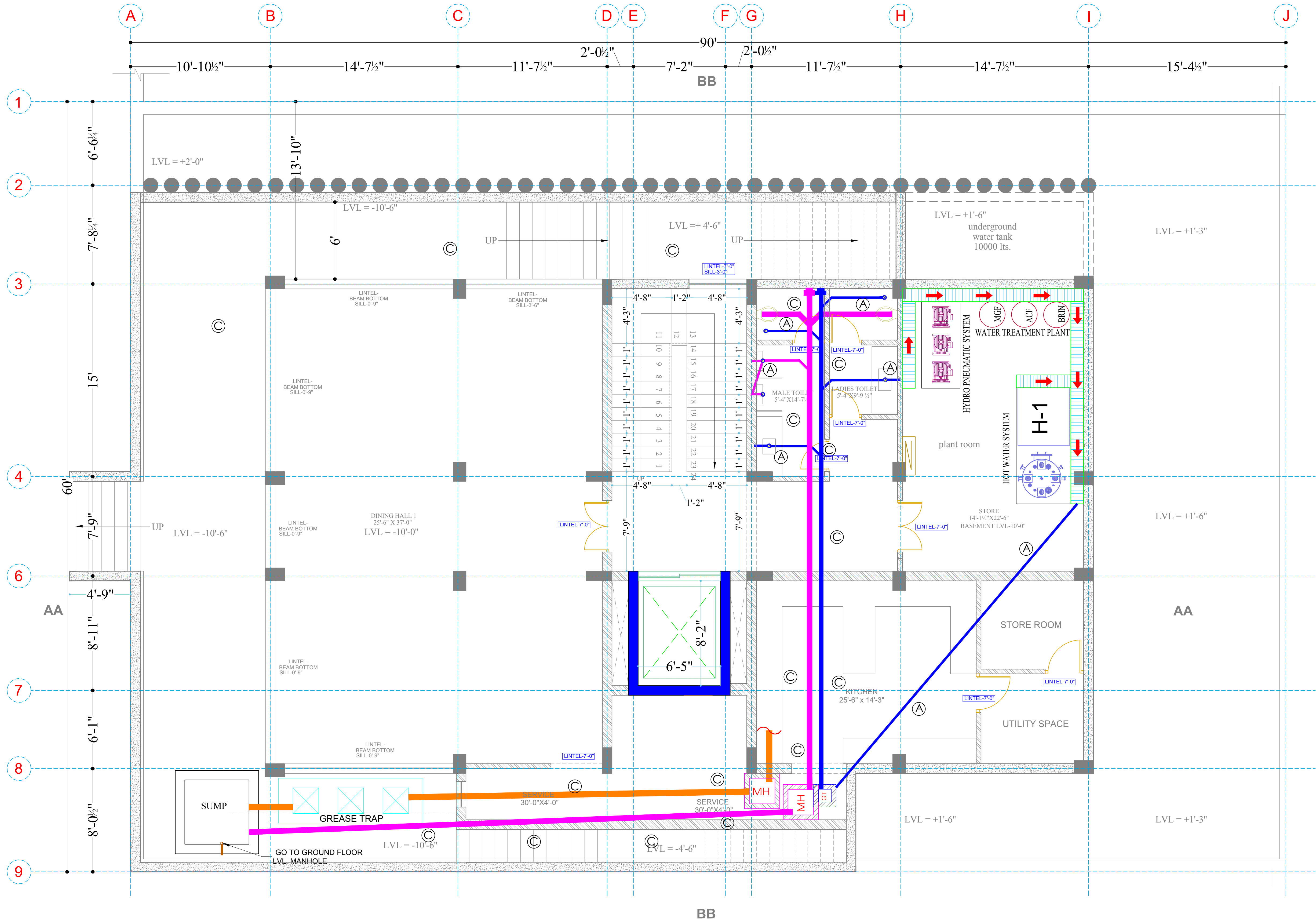
BASEMENT FLOOR
