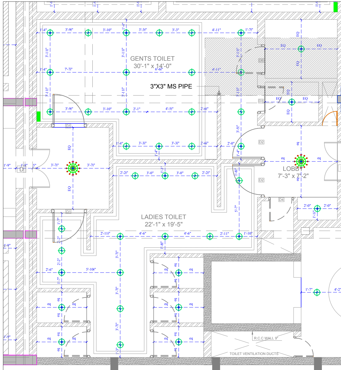
TOILET REFLECTED CEILING ELECTRICAL PLAN
