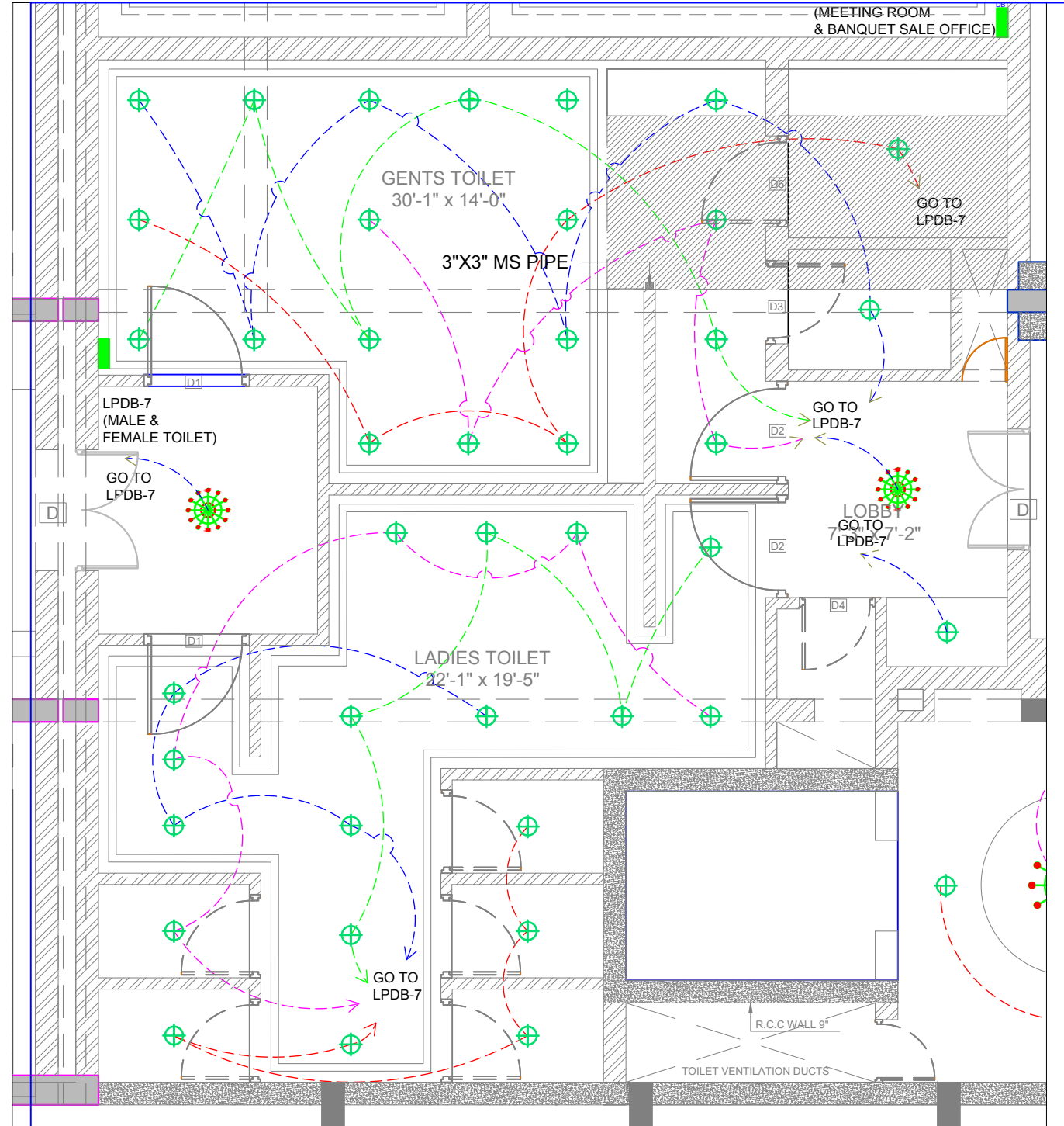
TOILET CEILING WIRE DIAGRAM
