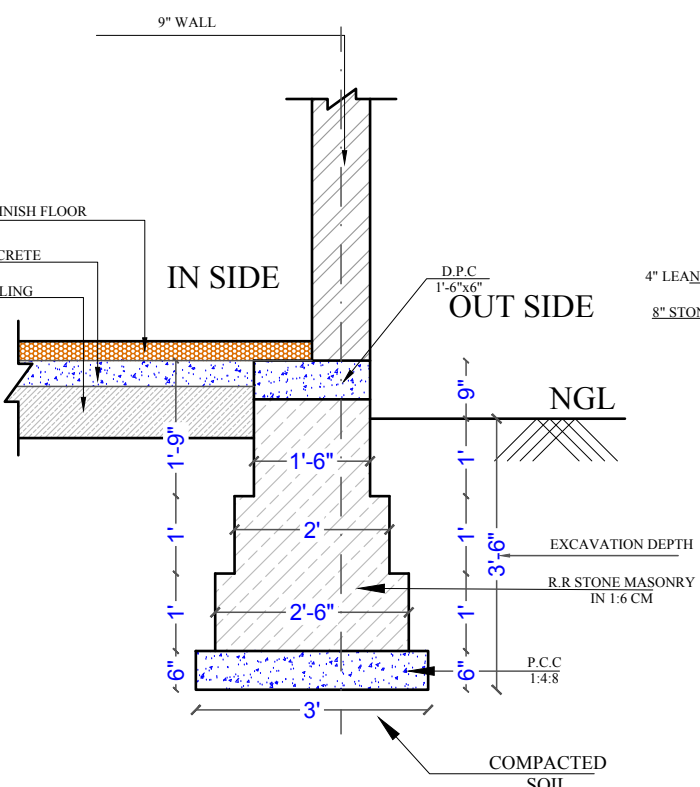
MASONRY FOUNDATION 9" OUTER LOAD BEARING WALL SECTION B-B
