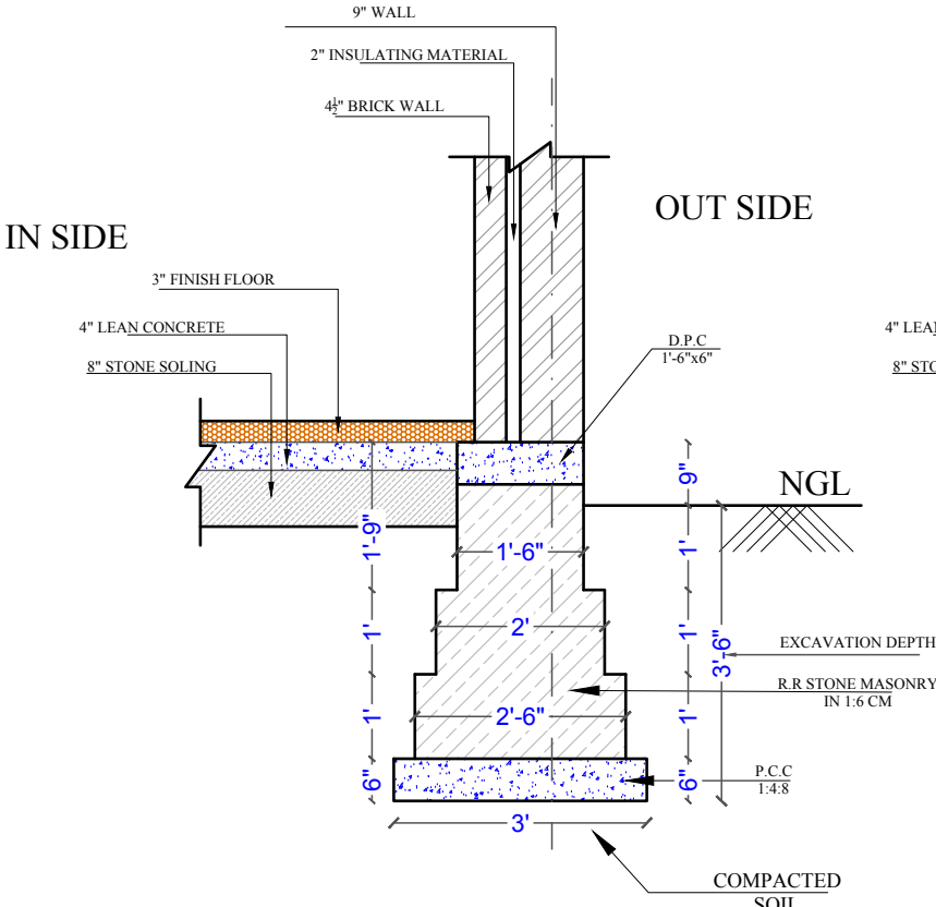
MASONRY FOUNDATION CAVITY WALL SECTION A-A
