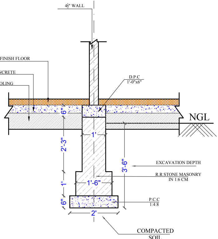
MASONRY FOUNDATION 4 1/2" INTERNAL PARTITION WALL SECTION D-D
