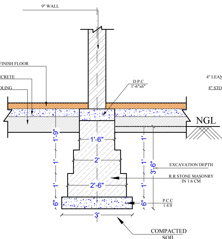
MASONRY FOUNDATION 9" INTERNAL WALL SECTION C-C
