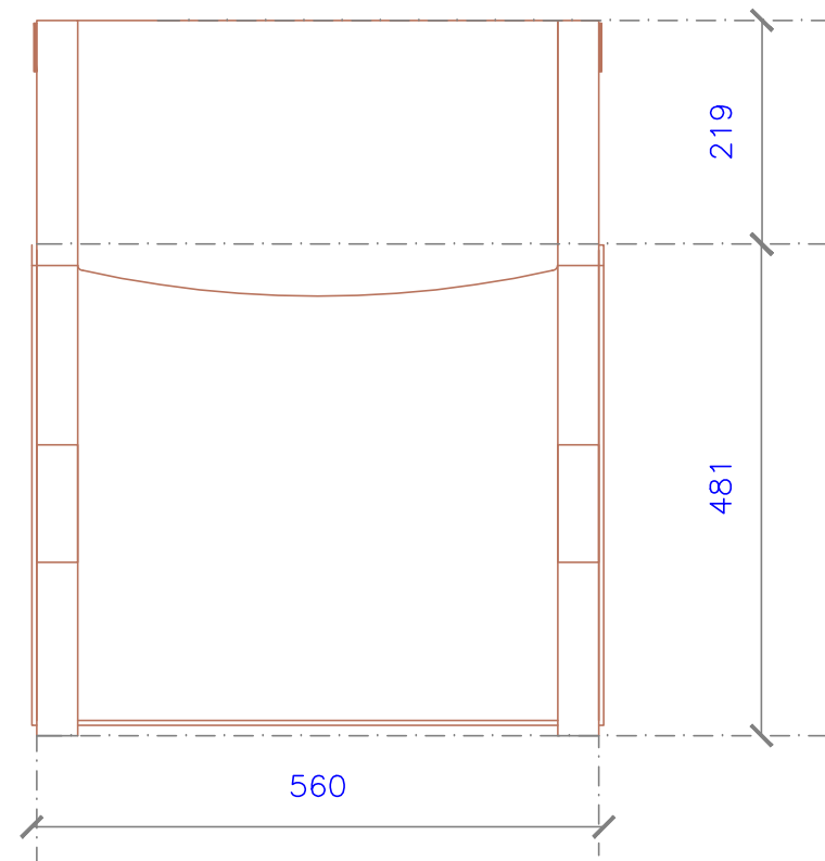
PLAN: STUDY CHAIR
