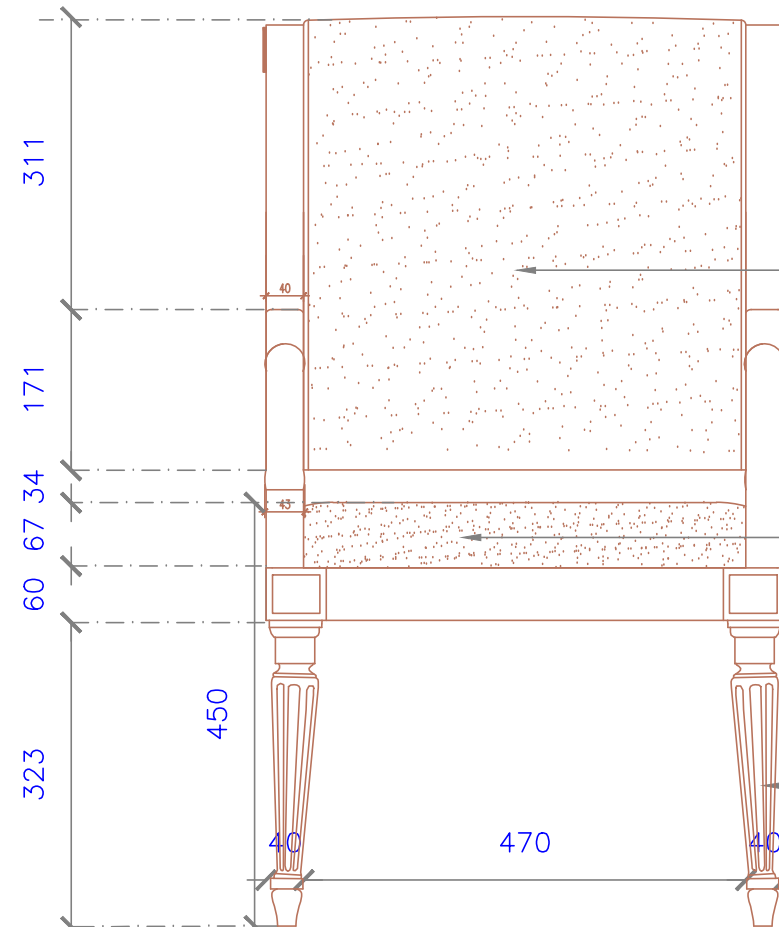
FRONT ELEVATION: STUDY CHAIR
