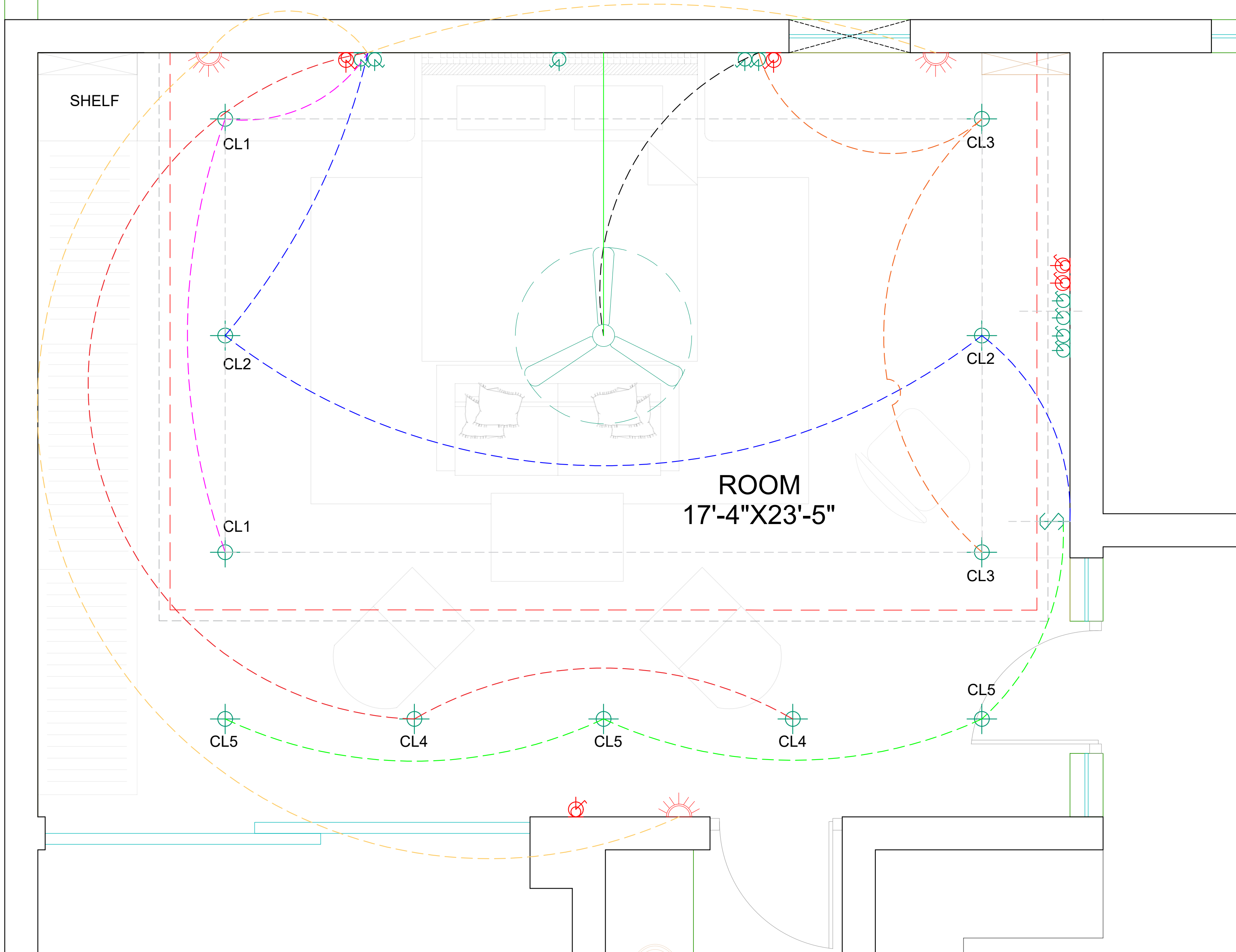
ELECTRICAL LAYOUT PLAN LOOPING
