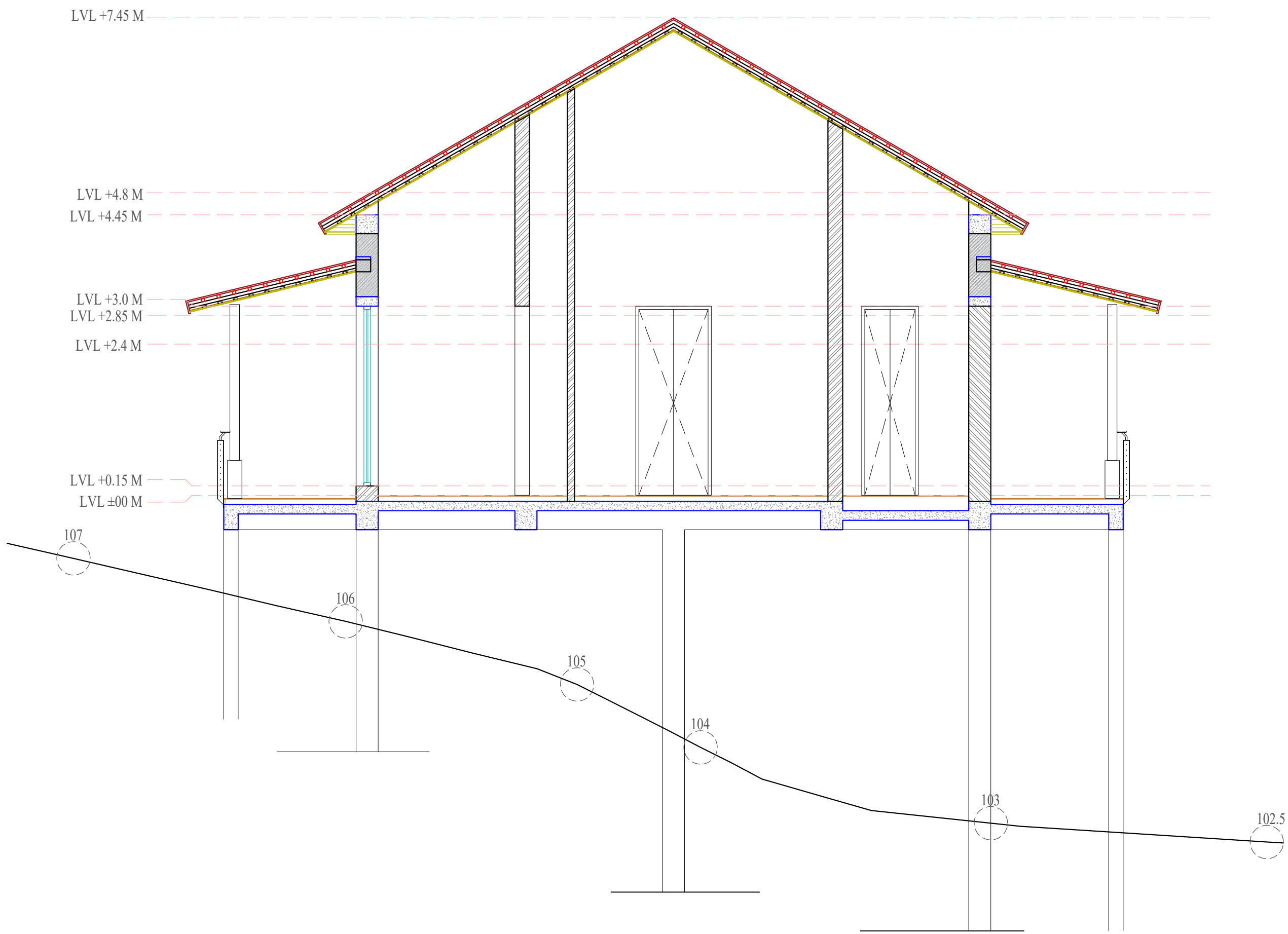
Section BB
