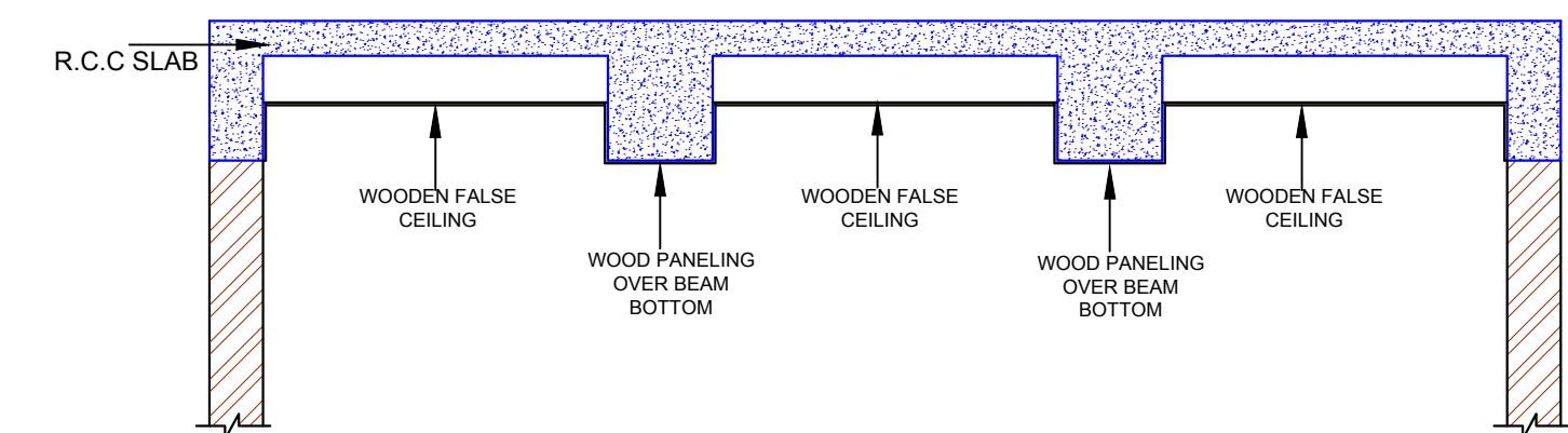
SECTION FROM MULTIPURPOSE ROOM
