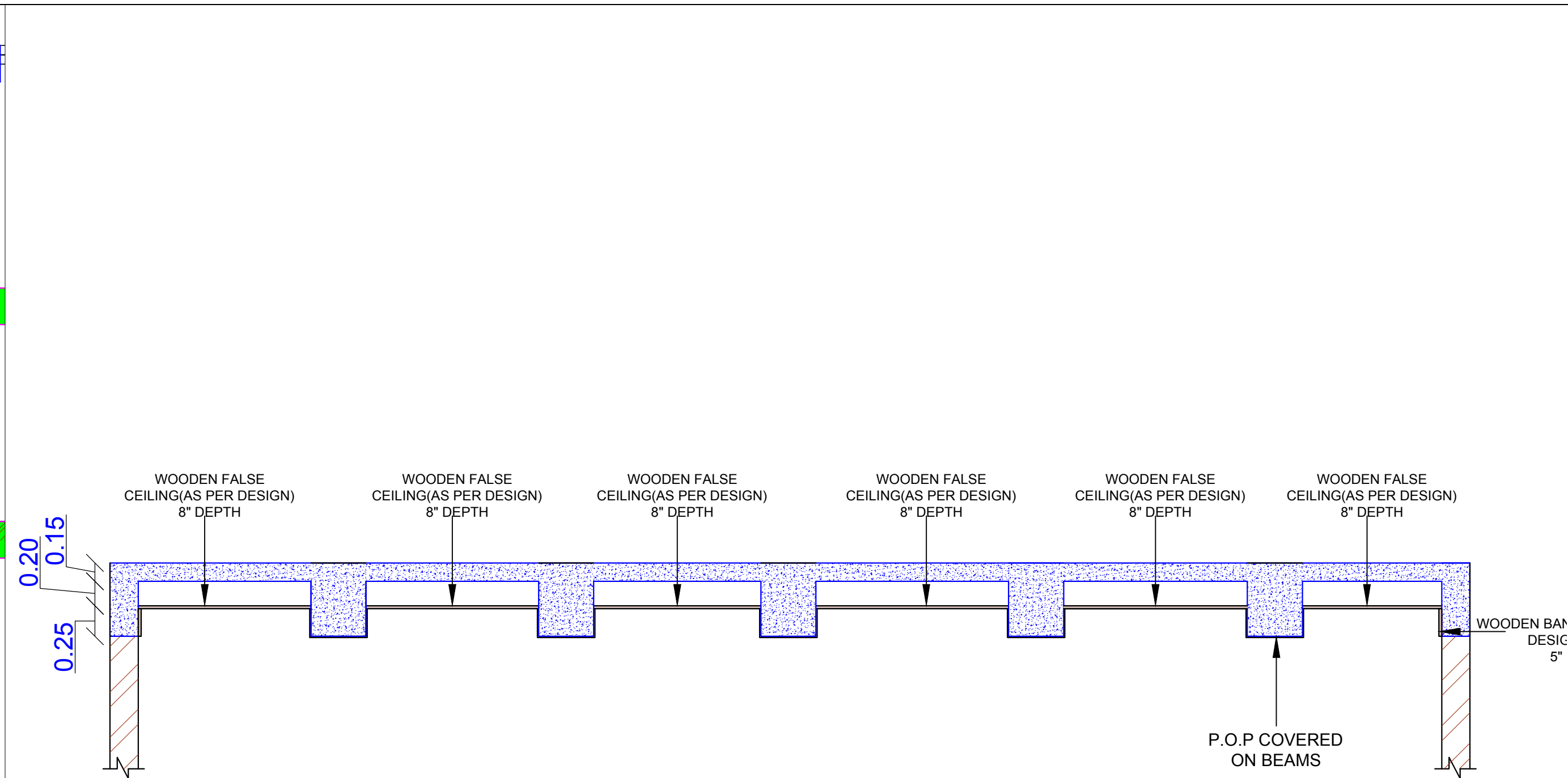
SECTION FROM CONFERENCE ROOM
