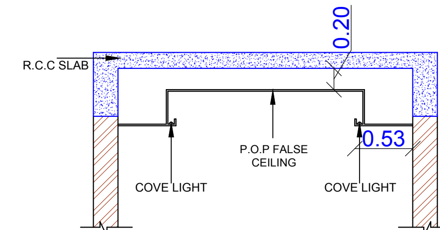
SECTION FROM CORRIDOR
