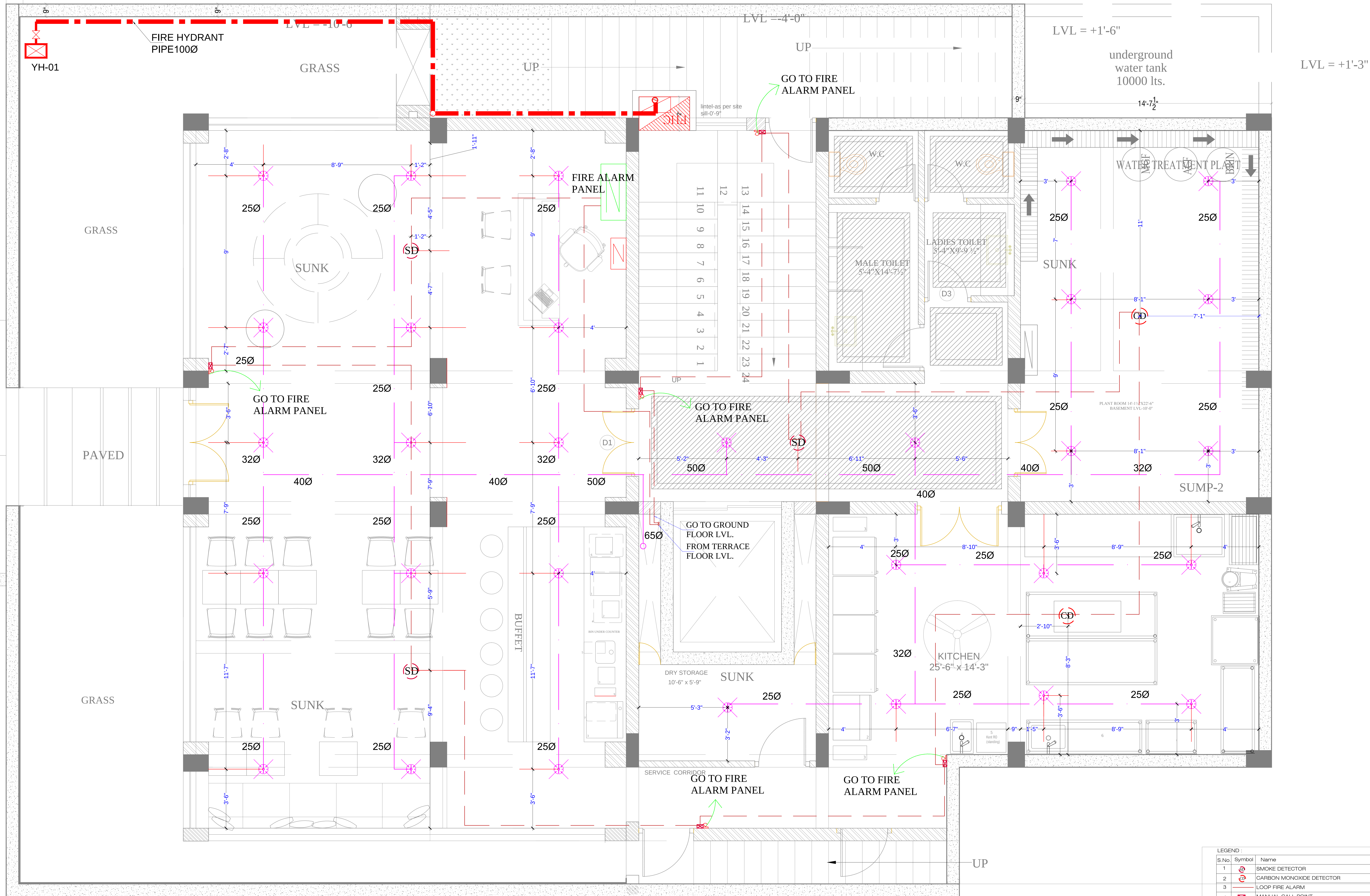
BASEMENT FLOOR
