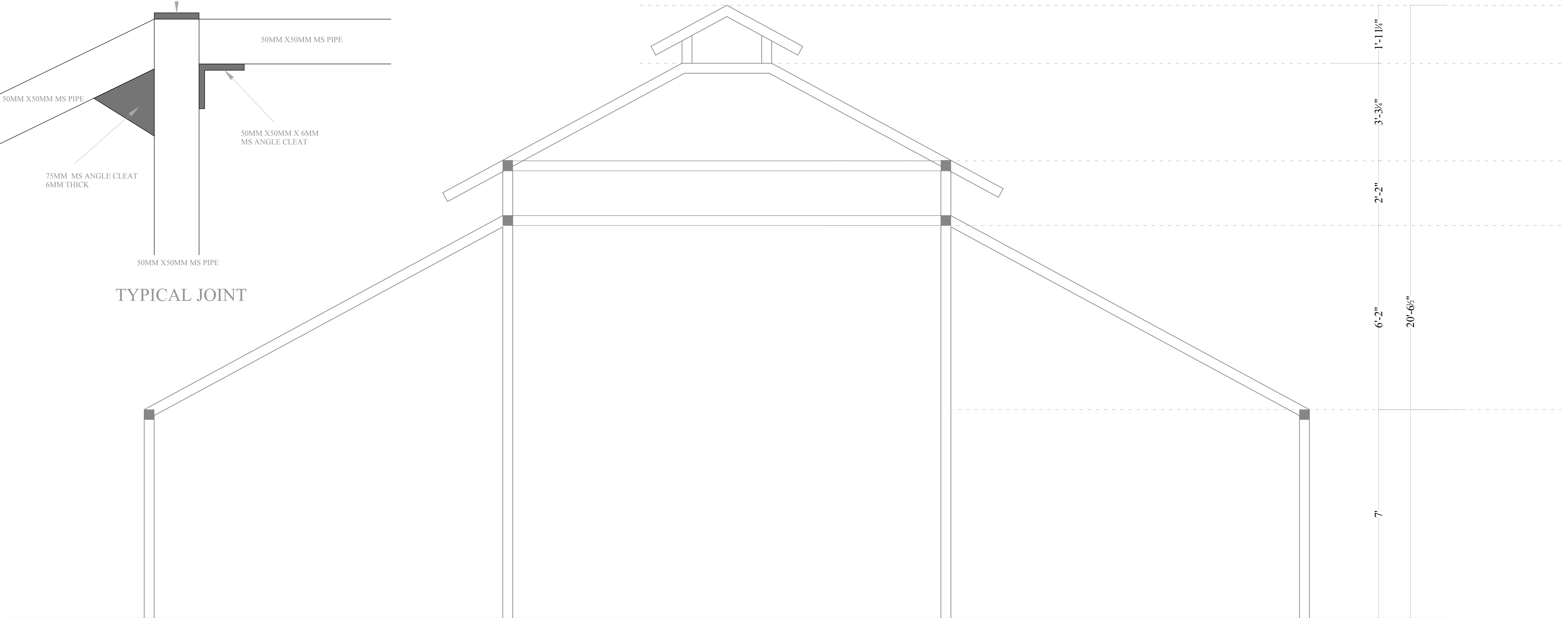
SECTIONAL ELEVATION
