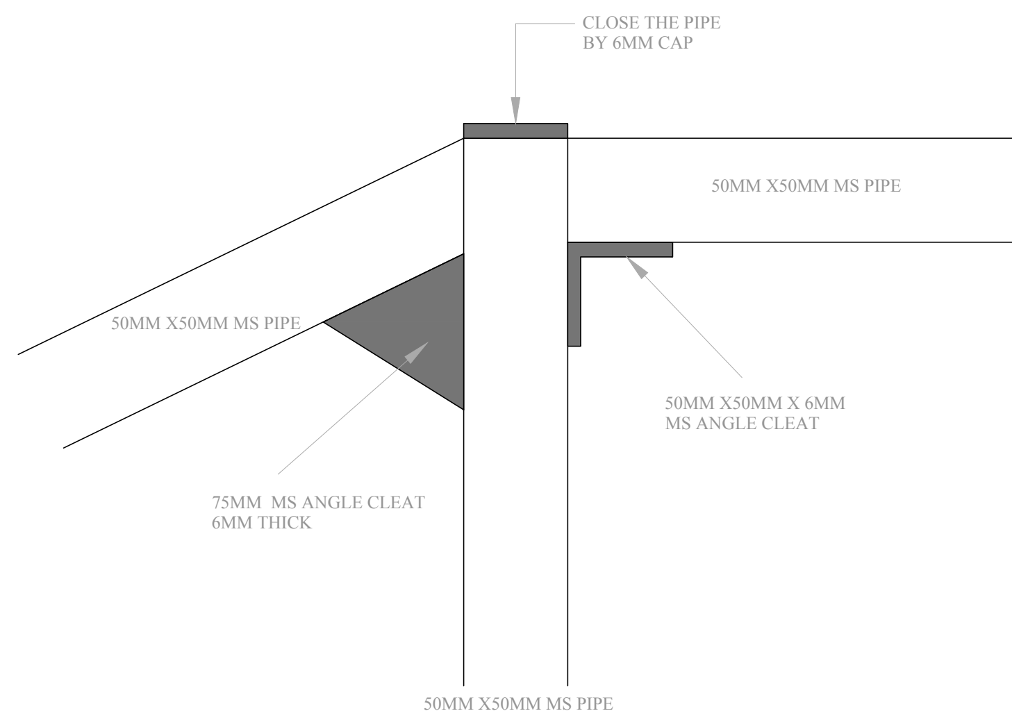
TYPICAL JOINT
