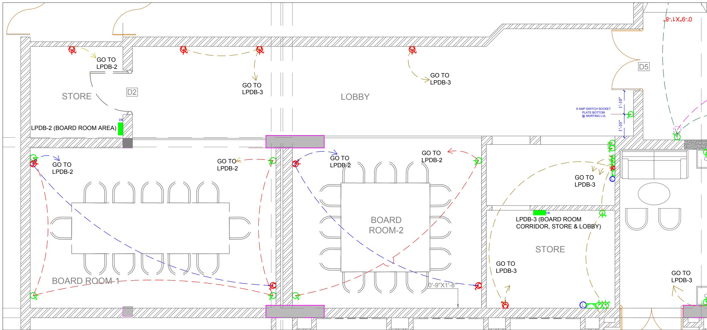
BUSINESS CENTER WALL WIRE DIAGRAM
