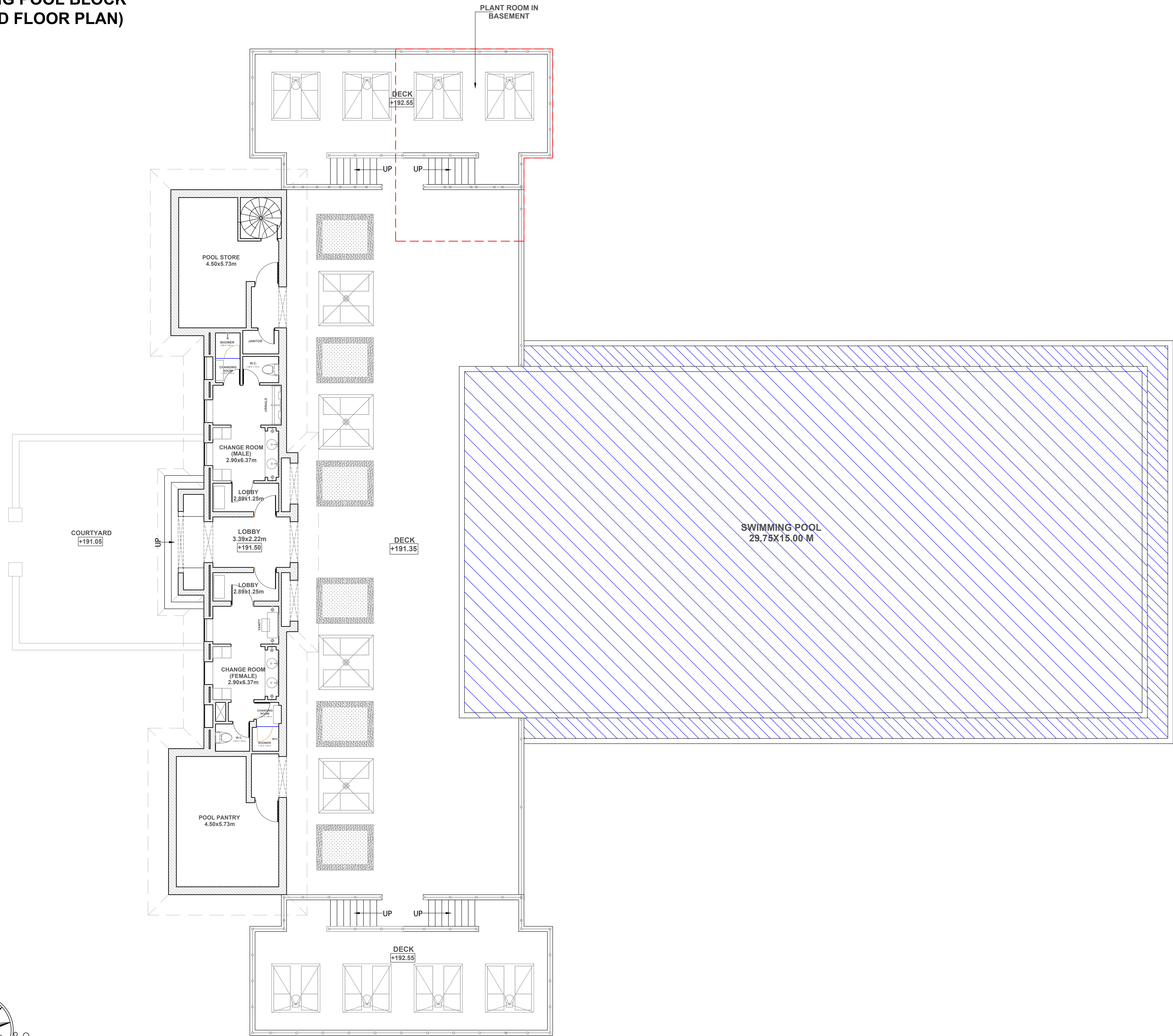
GROUND FLOOR PLAN SWIMMING POOL BLOCK
