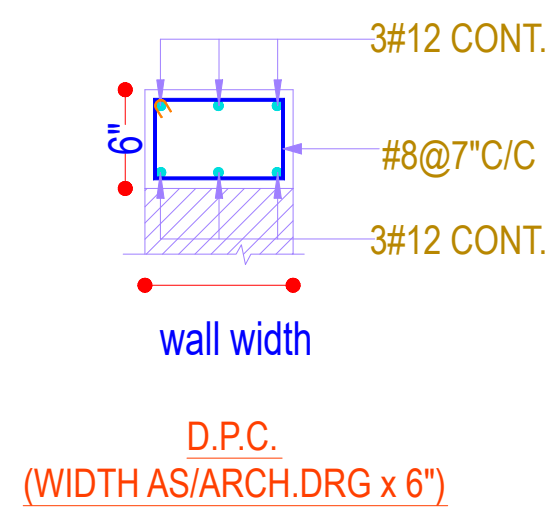
PARTITION WALL (SECTION-E)
