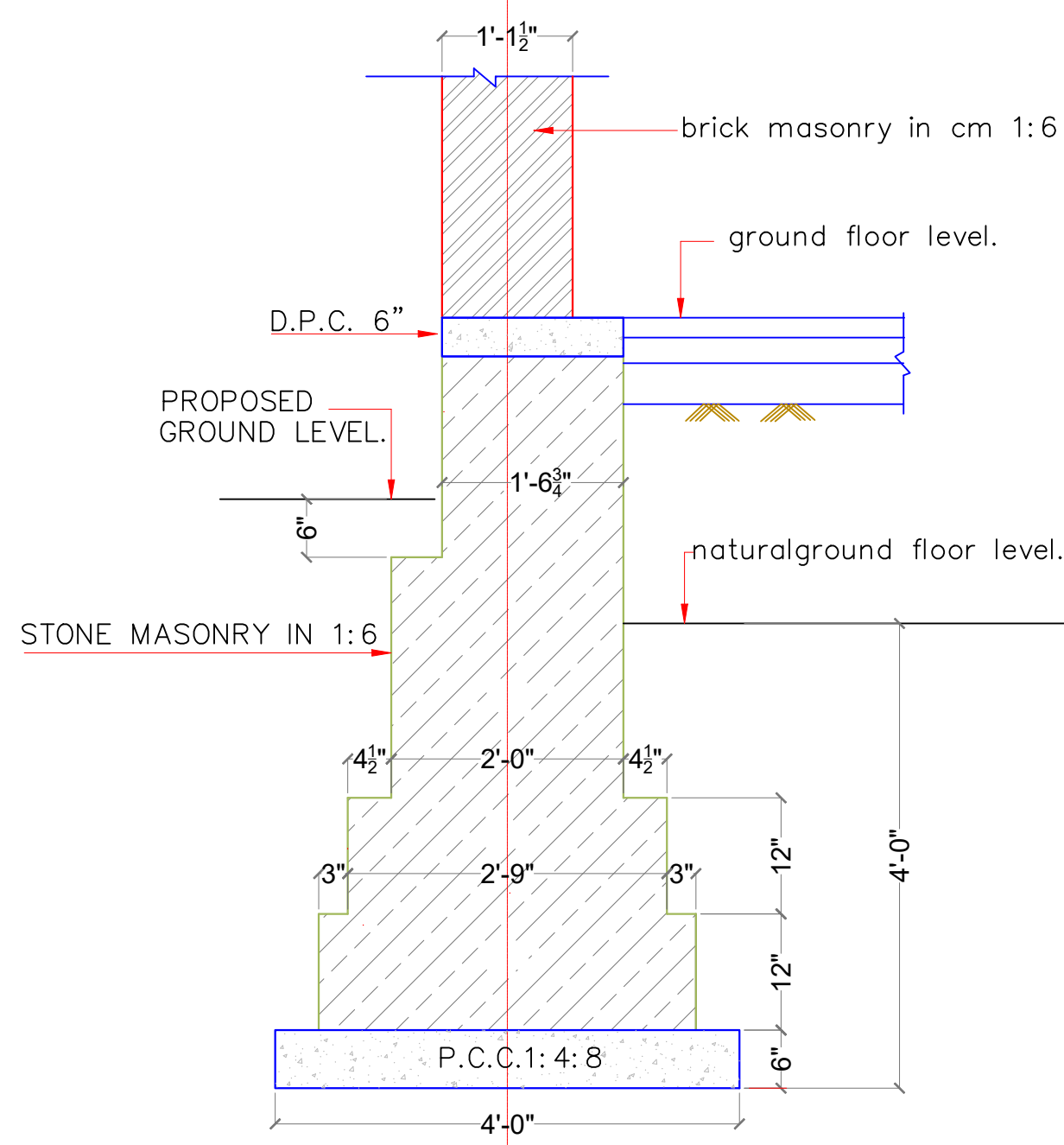
13.5 " OUTER WALL (SECTION-A)
