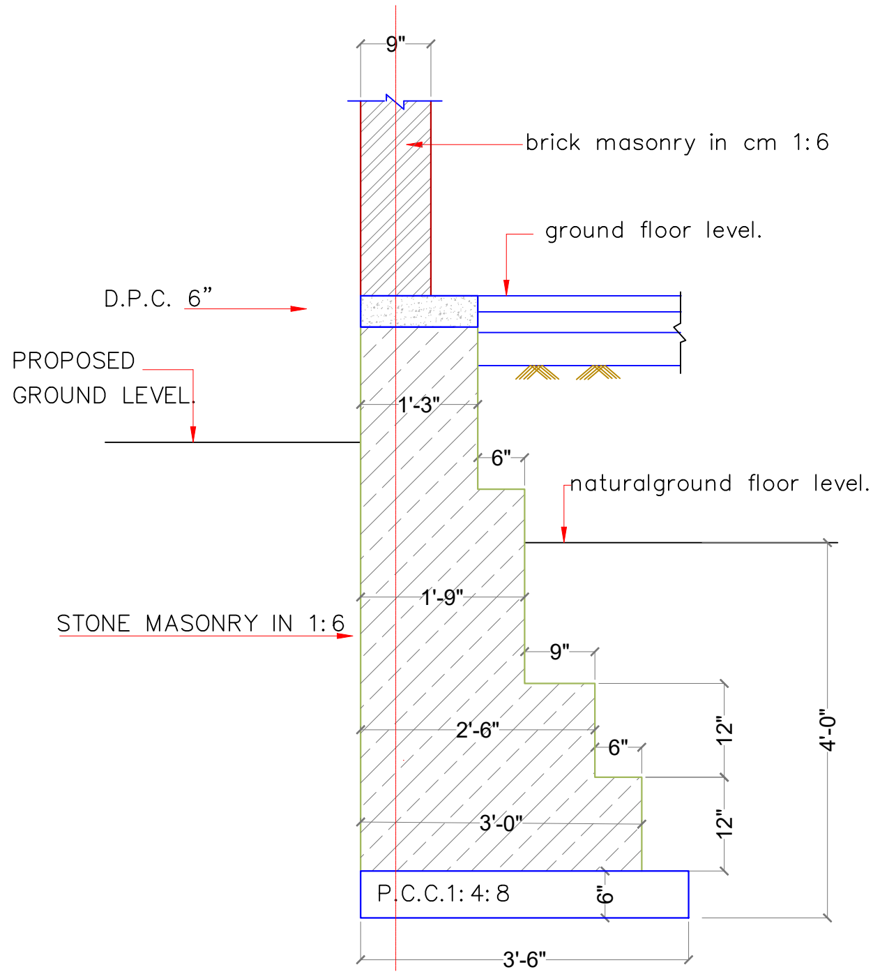
9" INNER WALL (AT EXPANSION JOINT) (SECTION-D)
