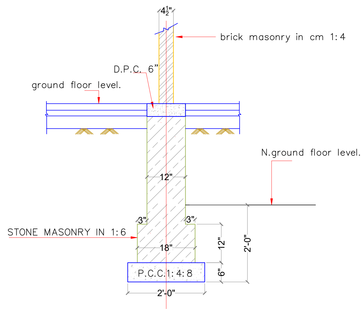
PARTITION WALL (SECTION-E)
