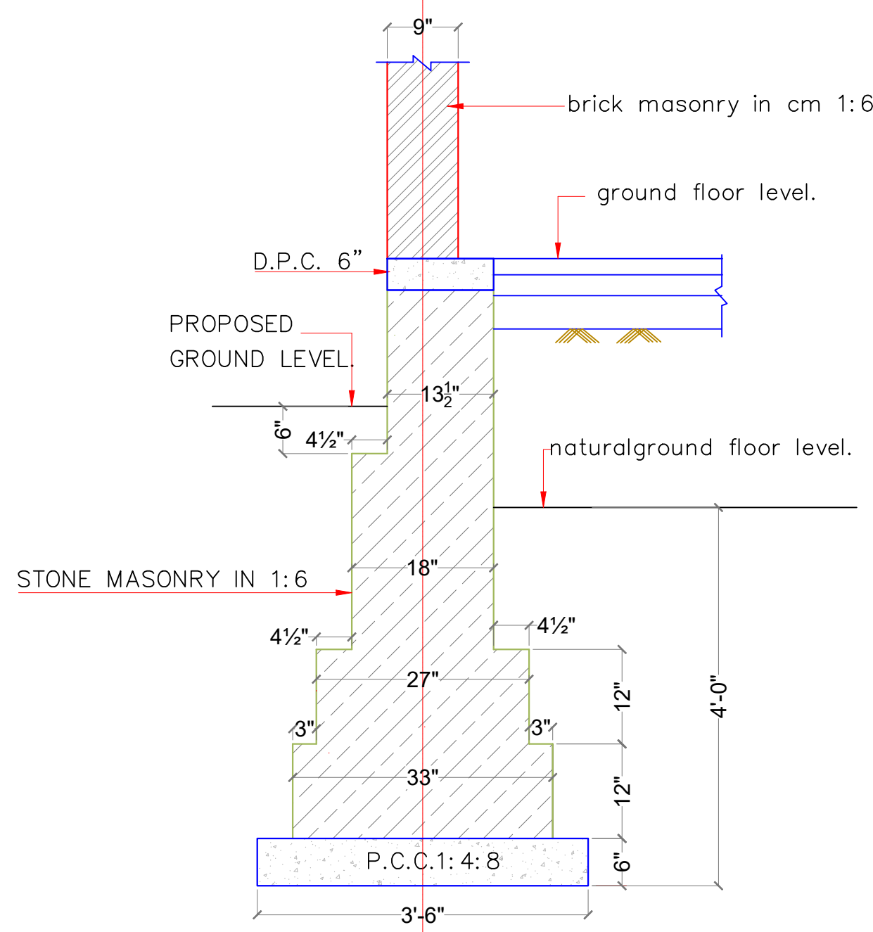
9" OUTER WALL (SECTION-B)
