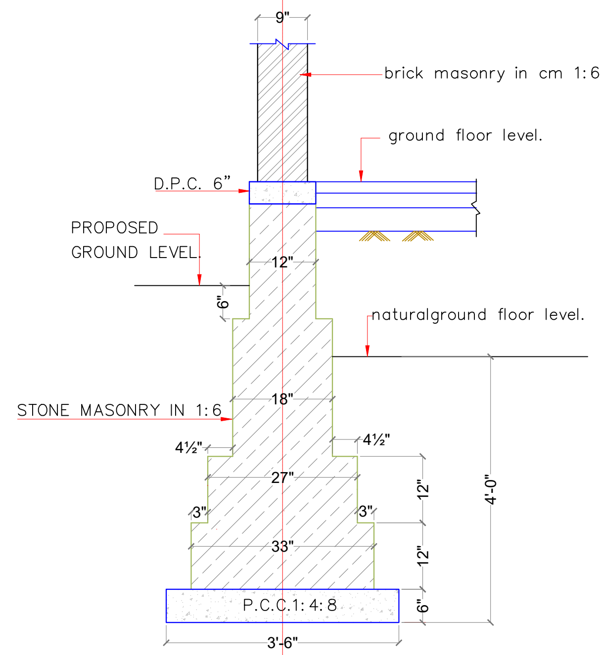
9" INNER WALL (SECTION-C)
