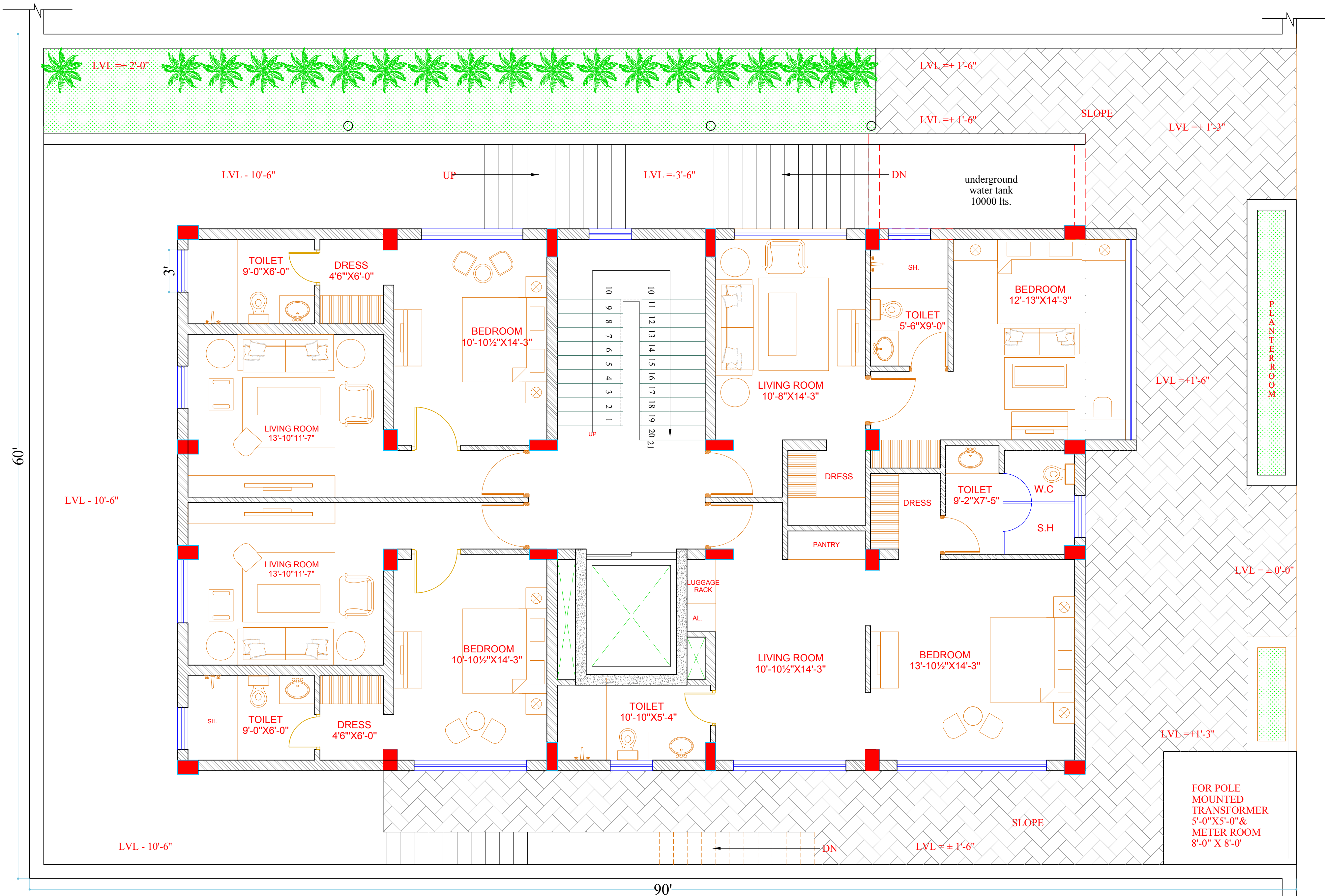
REVISED GROUND FLOOR
