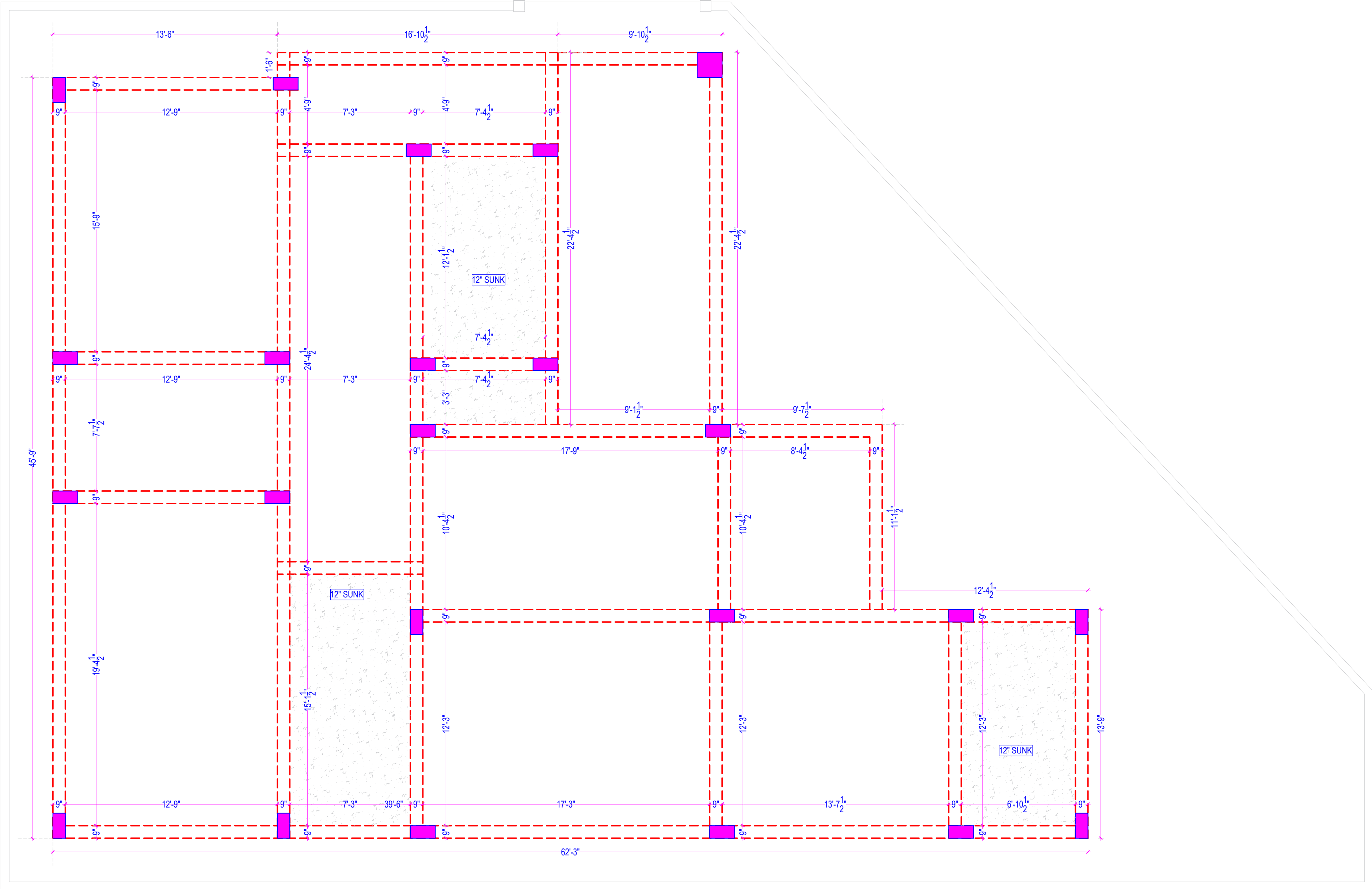
FIRST FLOOR SHUTTERING PLAN
